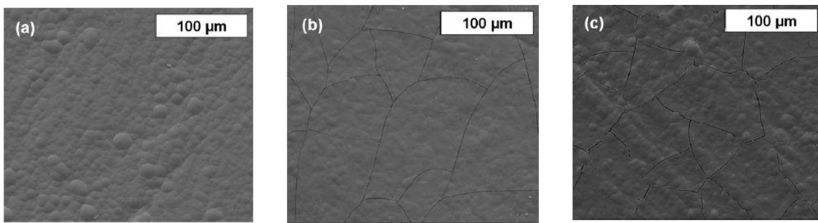
Figure 1.5. Scanning electron microscopy images revealing the typical surface morphologies of (a) Re–Fe, (b) Re–Co, and (c) Re–Ni alloys.
