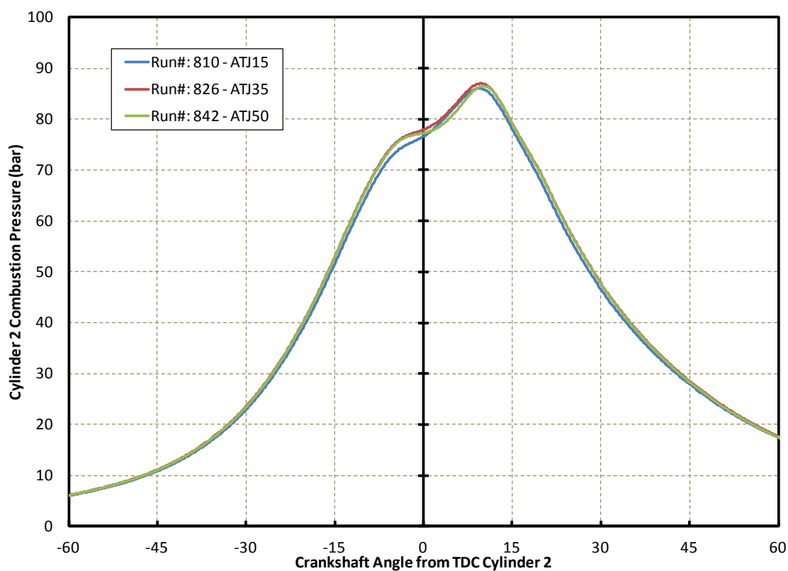
Figure 16. Main Chamber Pressure Histories for 3,400-RPM and 100% Load
