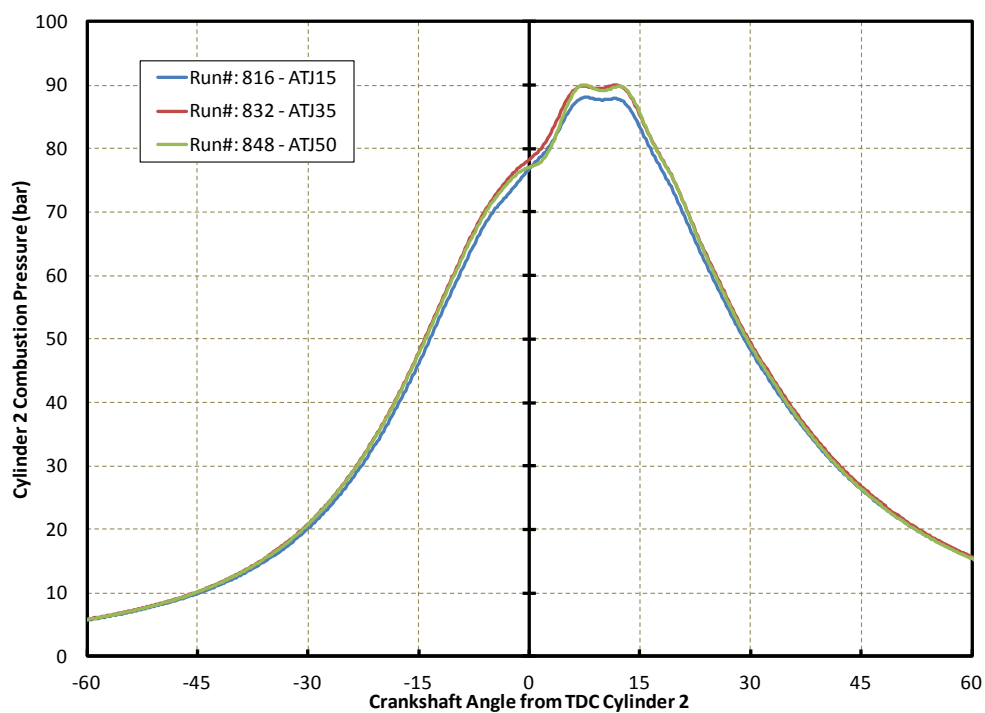
Figure A-14. Pre-Chamber Pressure Histories for 2,641-RPM and 75% Load, ESC4
