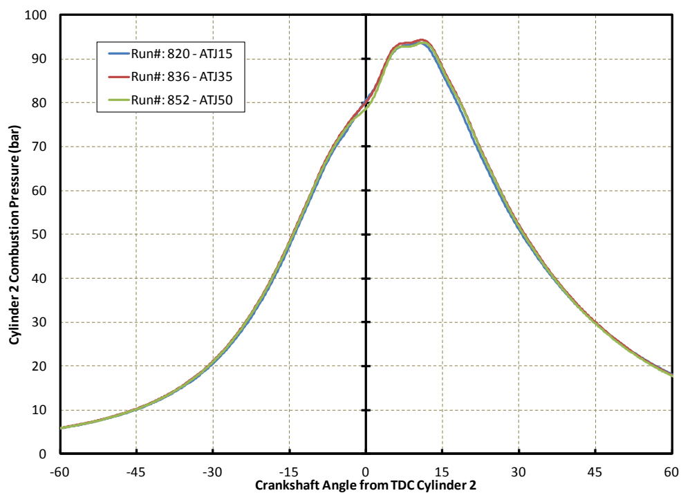
Figure A-30. Pre-Chamber Pressure Histories for 2,641-RPM and 100% Load, ESC8
