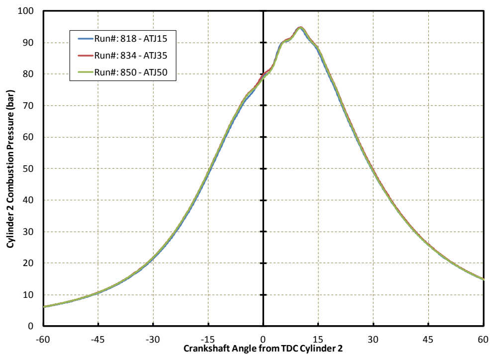
Figure A-22. Pre-Chamber Pressure Histories for 1,928-RPM and 75% Load, ESC6
