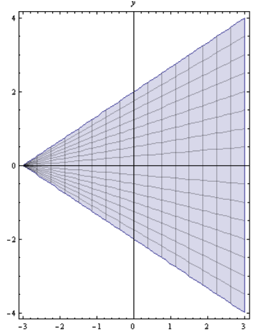
Figure 9.2.3: Graph of the BQ of (9.19) with \beta = 0.999 ( p' = -1.0010 ).
