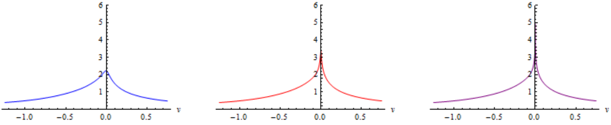
Figure 6.3. The integrand of (6.12) for the third BQ ( i.e. , with (6.18) substituted in it) as a function of v over the range of integration. From left to right: h = 0.1, 0.01, 0.00 . Though it is not clear from this picture, the function is singular at the origin when h = 0 .
