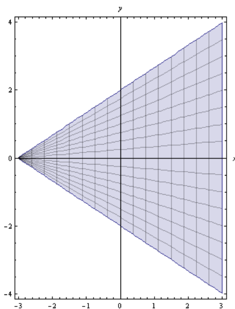
Figure 9.2.2: Graph of the BQ of (9.19) with \beta = 0.99 ( p' = -1.0101 ).
