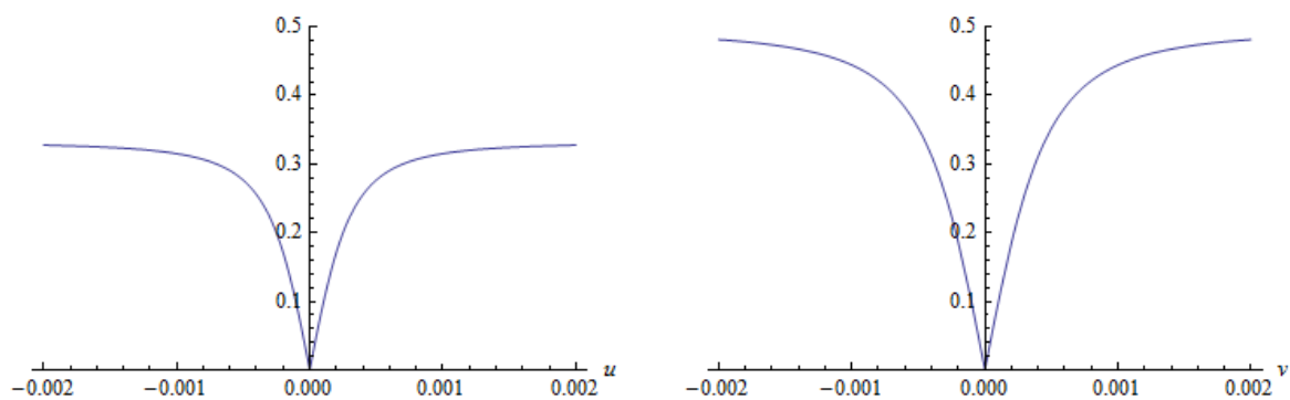
Figure 4.7.2. Graph of the integrand \rho / R for h = 0.1 along v = 0 (left) and u = 0 (right) for the second BQ of Section 3. The origin is the point (4.16).
