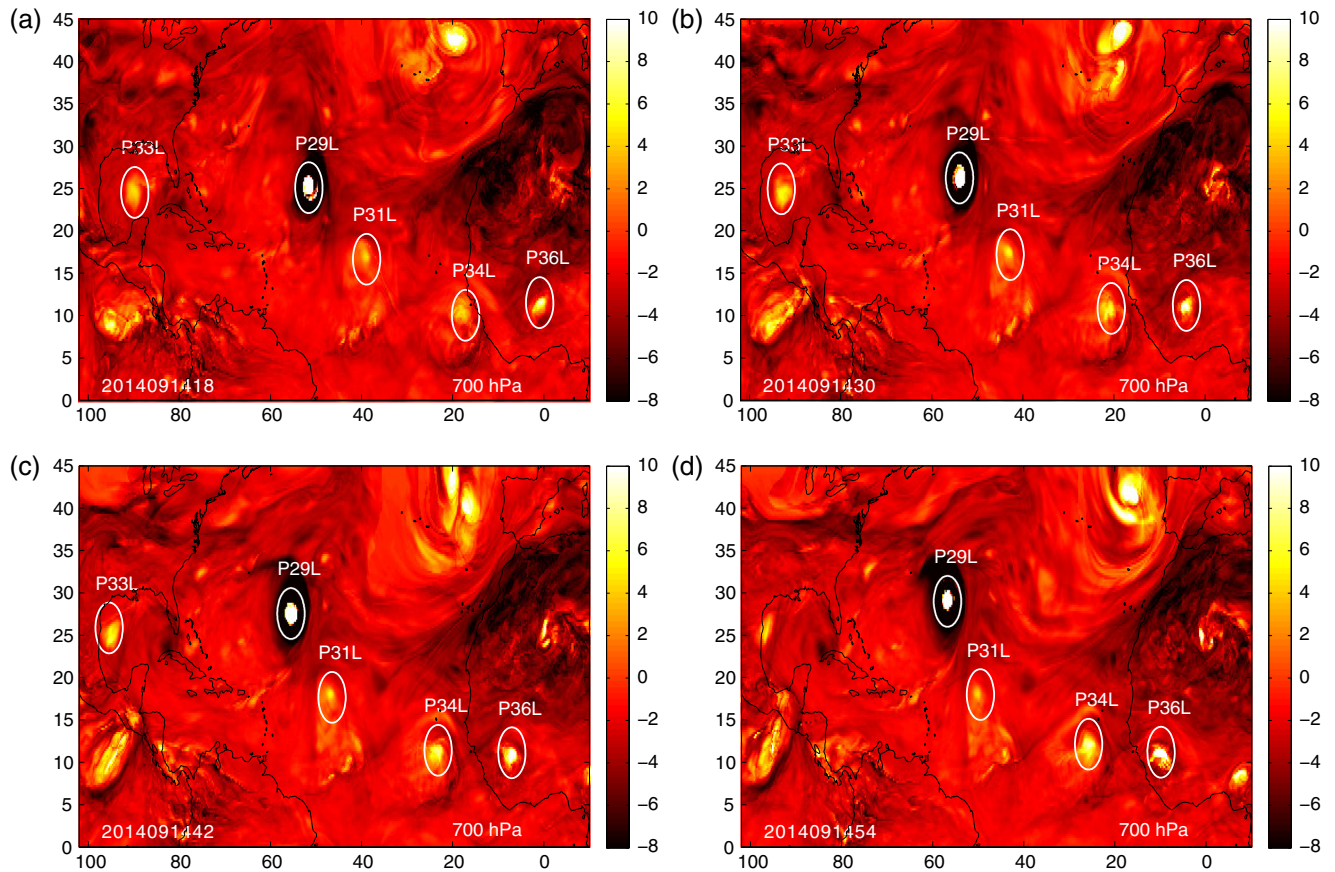
Figure 5. The time evolution of the OW_{Lag} field for the Atlantic development region on 14 September at forecast times of (a) +18 h, (b) +30 h, (c) +42 h, and (d) +54 h.
