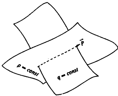
Figure 1. Intersection of surfaces of \rho and q (from Chu 1995, Marine Technology Society Journal).
