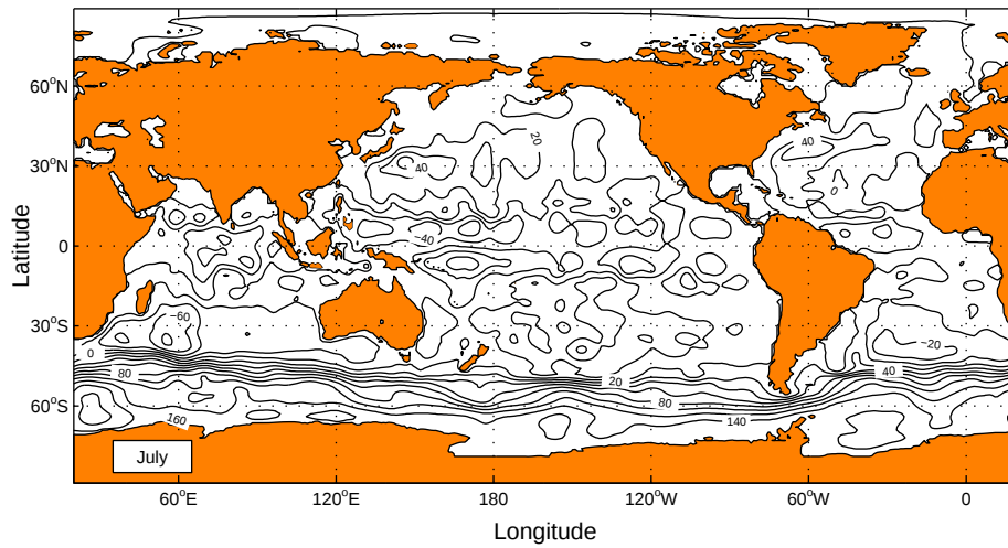
Figure 3. Inverted global volume transport stream function (unit: Sv): (a) annual mean, (b) January, and (c) July (from Chu and Fan 2007, Journal of Marine Systems ).
