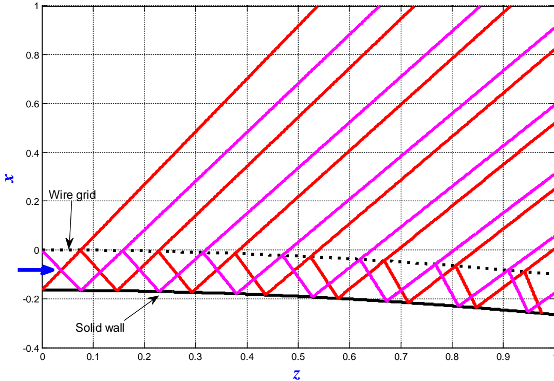
Figure 6. Departure from parallel-ray outputs due to the curved walls.
