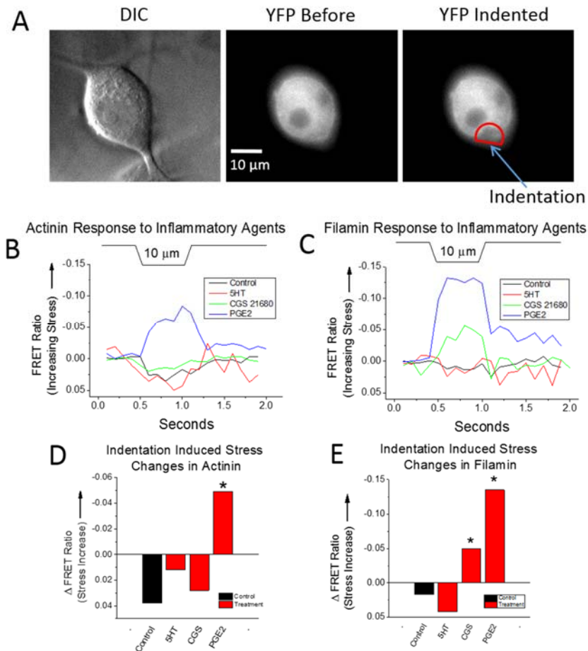
Figure 10. Inflammatory agents cause changes in the cytoskeleton sensitivity to stress. DRGs transfected with cpstFRET chimeras of actinin and filamin were indented with a blunt glass probe – tip \sim 3 -4 \mu m diameter. The cell were indented \sim 10 \mu m with a trapezoidal shaped 0.5 sec long stimulus, a depth that produced maximal MSC currents in whole-cell recordings. (A) Shows a DIC image of a DRG soma, and the YFP fluorescence images before and at the peak of the indentation to show the change in distribution of the stress probe. The red semicircle outlines the region of the interest (ROI) used to analyze the FRET changes during indentation. Cells were indented 9 times before and during treatment with inflammatory agents, and the signals averaged. Images were acquired at a rate of 10 frames/sec. The mean response from 15-20 cells was averaged in the ensemble responses shown in (B and C). The FRET response was measured before (black control traces) and after 20-60
