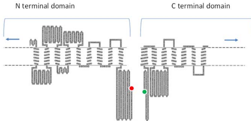
Figure 4 Two PIEZO1 fragments when coexpressed produced an active channel. This construct allows access to internal transmembrane domains where we can delete sequences to produce smaller channels. Fluorescent tags are indicated by colored circles.
