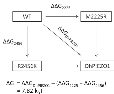
FIGURE 6 Mutant cycle analysis. The energy difference between open and inactivated states for WT, single-site mutants, and DhPIEZO1. The free energy change in DhPIEZO1 ( \Delta\Delta G_{DhPIEZO1} ) is larger than the sum of free energy changes for the two single mutants by \sim 8 \text{ k}_B\text{T} , showing that the sites are not independent but exhibit positive cooperativity.
