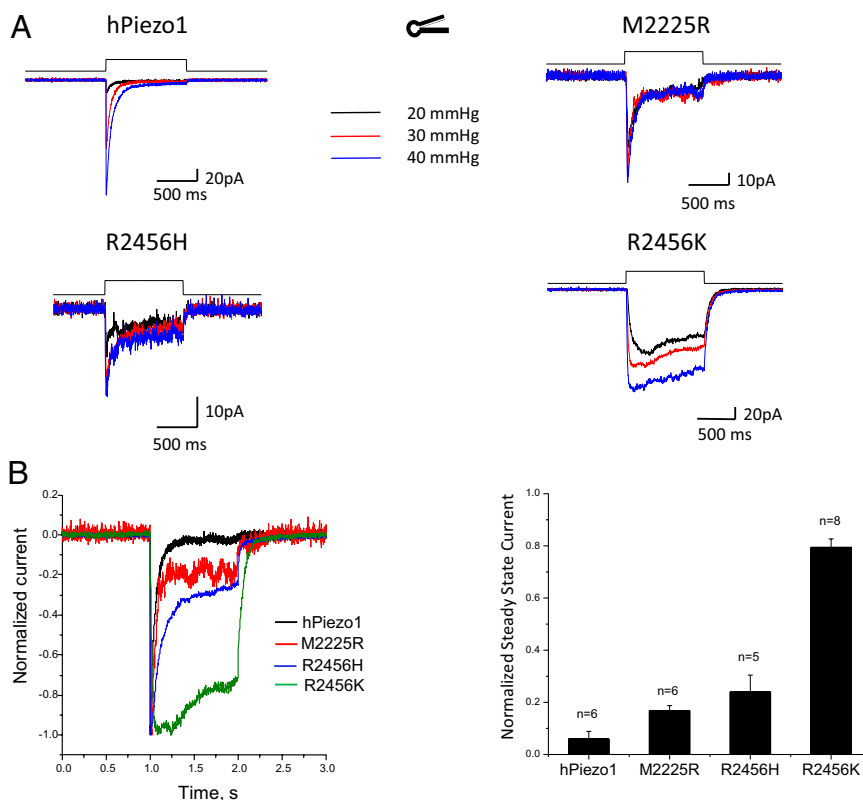
Fig. 6. Response of O/O patches. ( A ) The difference between WT and mutants. M2225R and R2456H have partially restored inactivation; R2456H remains slow; R2456K does not inactivate at all. ( B ) The traces normalized for kinetic comparison. The ratio of peak to steady-state current (bar graph with SD) illustrates that, even with the partial restoration of inactivation, M2225R and R2456H transfer more permeant charge than WT during an opening because of the longer open time. Deactivation (closure upon release of stress) was fast in patches from WT but was slow in mutants.
