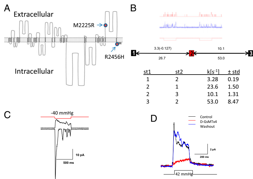
Fig. 1. Characterization of cloned hPIEZO1. (A) A diagram showing the putative transmembrane domains of hPIEZO1 and intracellular and extracellular regions. The HX mutation sites are shown where M2225R is thought to be extracellular and H2456 is intracellular. (B) Kinetic data and a fitted model for hPIEZO1 with three states (closed-open-inactivated). The theoretical fit to the model shown in red provided the kinetic rate constants shown in the table. The pressure dependence is shown in parenthesis. (C) Voltage-dependent inactivation. At depolarized voltages (+40 mV) there is slow inactivation, and at hyperpolarized voltages (−110 mV) there is rapid inactivation. (D) hPIEZO1 is inhibited by the D enantiomer of GsMTx4 (2 \mu M, +50 mV holding potential).
