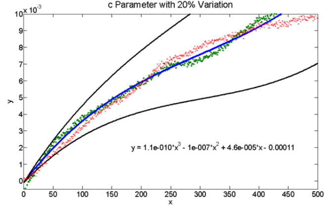
Figure 6: Performance degradation plots. Two examples showed (darker dots, lighter dots). Third order model fit to data. 20% Bounds on \mathbf{c} parameter shown by black lines.
