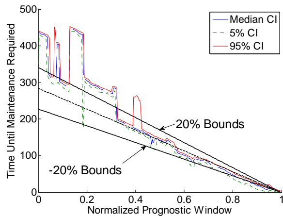
Figure 10: Alpha-Lambda Performance with 20% error bound. Prediction until MIR showing Median, 5%, and 95% confidence levels (CI).
