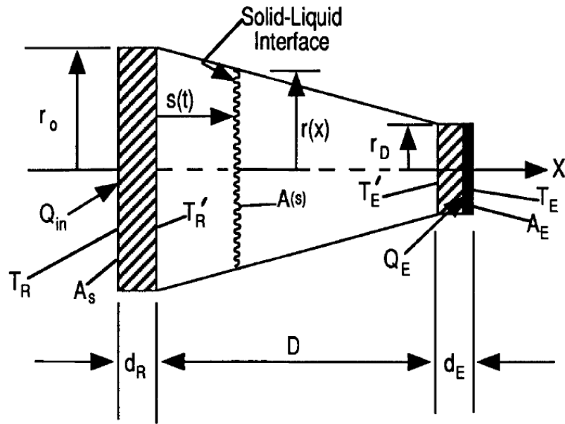
Figure 4.9: Diagram of the silicon freezing model proposed in Chubb et al [5]. Note the large receiver area ( A_s ) and small emitter area ( A_E ) which are intended to smooth thermal gradients during the freezing process.
