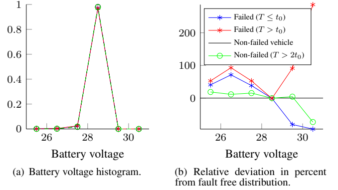
Figure 10. Histogram for variable BattVoltTempI3, i.e., battery voltage when the battery temperature is in the range of 10 to 25°C.
