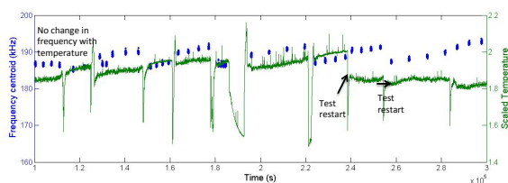
Figure 12. The comparison of AE data with gearbox FWD load.
