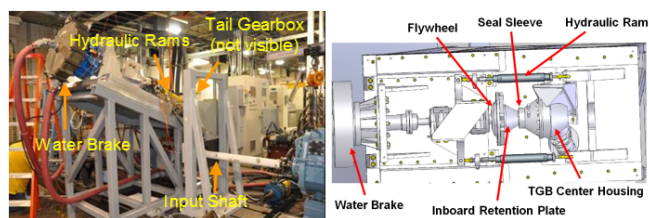
Figure 1. The experimental test stand.
