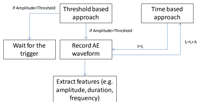
Figure 3. The comparison of threshold-based and time-based approaches.
