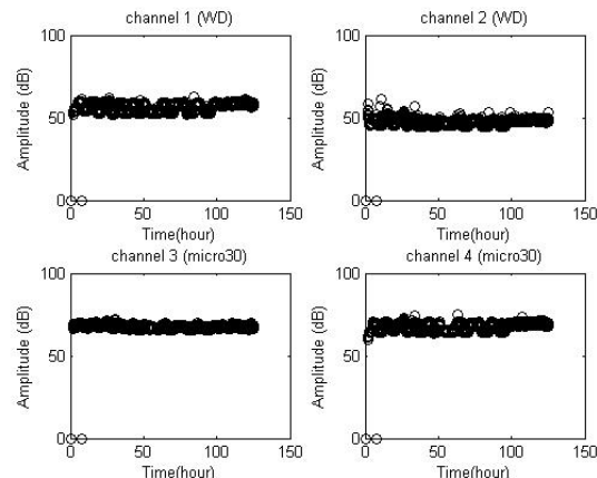
Figure 6. Amplitude histories of AE sensors over 130 hours testing.
