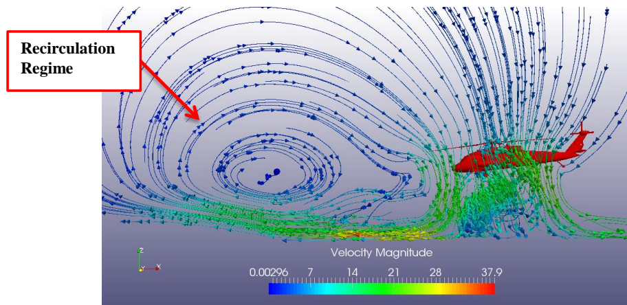
Figure 4 – Re-Circulation Flow in Low Speed Acceleration Near the Ground
