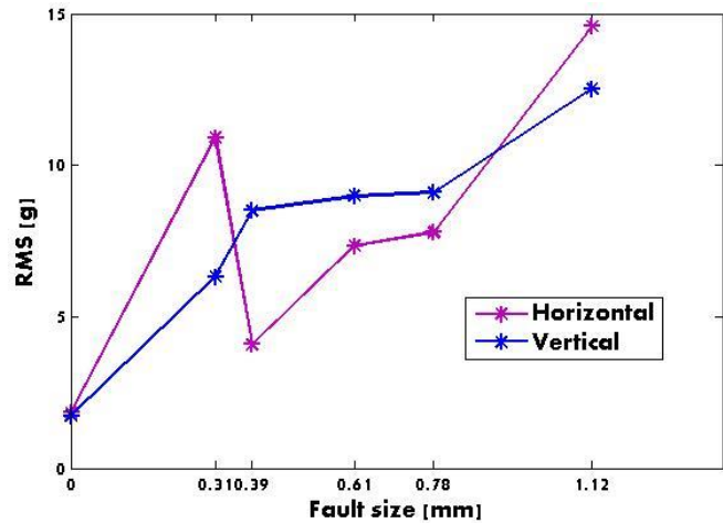
Figure 12. Experimental results of acceleration RMS vs fault size when fault located 90° to the loading zone (location “B”).
