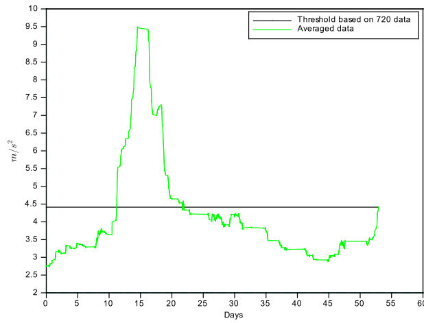
Figure 9. Averaged HFBP data over time with threshold based on fitting Johnson distribution with 720 averaged data in power class 2.
