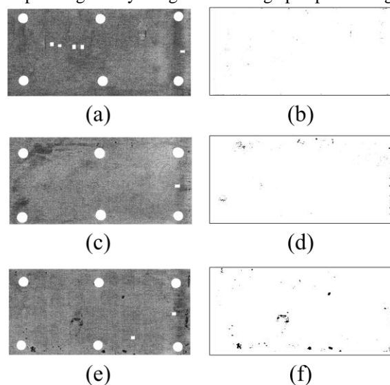
Figure 12. Whole panel image pre-processing. Left column: intermediary images with rivet holes and marked numbers whitened of (a) Panel 1 with 133-hr corrosion exposure, (c) Panel 2 with 209-hr corrosion exposure, (e) Panel 3 with 286-hr corrosion exposure. Right column: binary images after pre-processing of (b) Panel 1, (d) Panel 2, (f) Panel 3.
