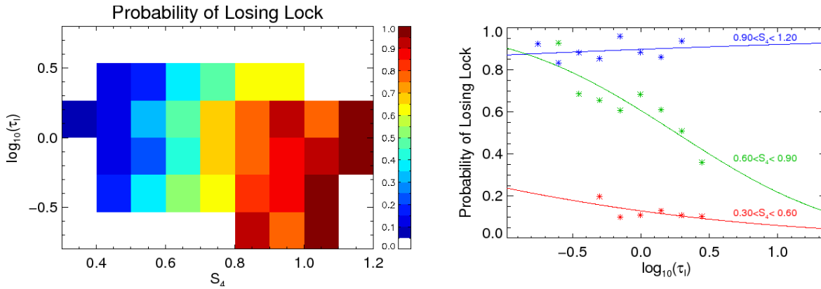
Figure 34. Probability of Losing Lock versus both S_4 and \tau_1 (left); Probability of Losing Lock versus \tau_1 for three Different Ranges of S_4 Values (right)
