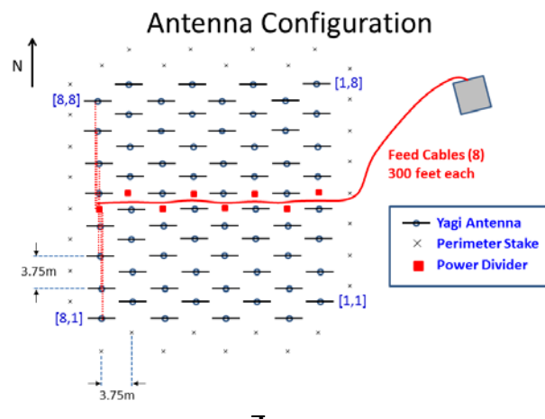
Figure 59. Blue Nile Radar Antenna Configuration
