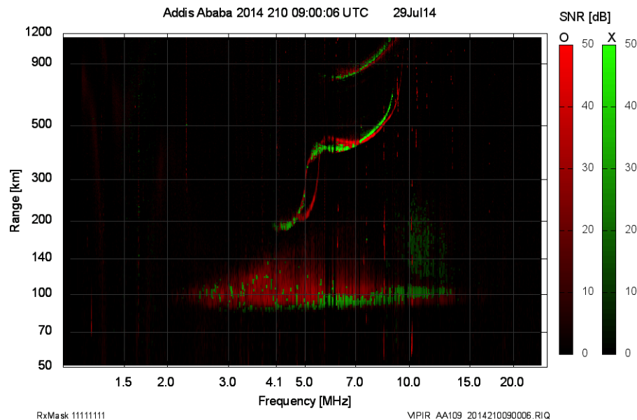
Figure 55. Ionogram Recorded by Addis Ababa VPIR Ionosonde on July 29, 2014
