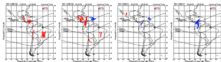
Figure 3. MSTID's Phase Velocities Calculated using the Cross-Correlation Method (CCM)
