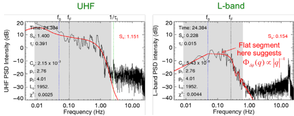
Figure 43. Measured Intensity Spectrum (black) and Least-Squares Fit by the Strong Scatter Model (red) for UHF and L-band at 24.38UT
