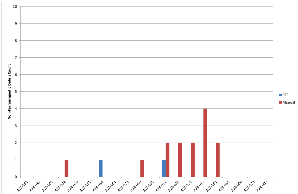
Figure 25: Comparison of Manual (red) and FST (blue) detection of non-ferromagnetic debris
