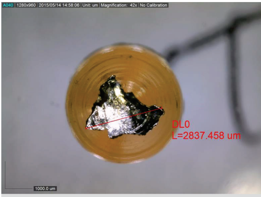
Figure 21: Flake X (real Fe wear debris) encapsulated in resin and used for FST testing
