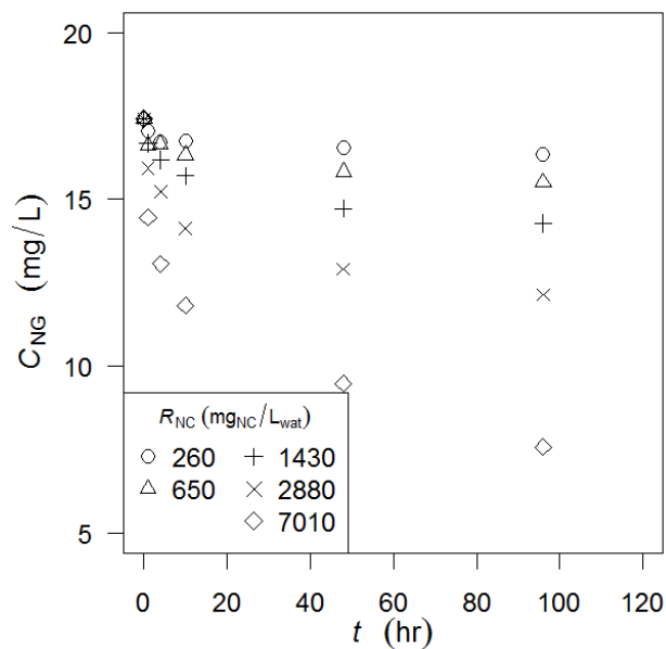
Figure 92. Sorption kinetic profile of NG to nitrocellulose. Aqueous phase NG concentrations were measured at different times in a batch sorption system at five different nitrocellulose-to-water ratios ( R_{NC} = 260, 650, 1430, 2880, \text{ and } 7010 \text{ mg}_{NC} (\text{L}_{\text{water}})^{-1} ).
