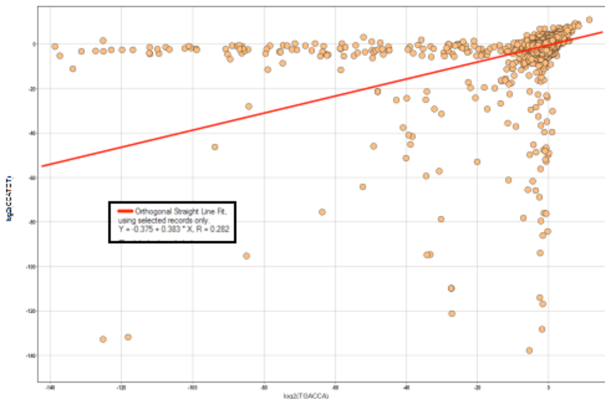
Figure 7. Correlation of mapped RNA-Seq transcripts of DCIS#007 with HTA2.0 array.
