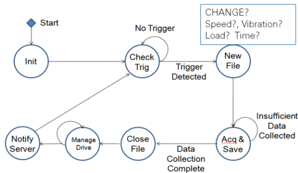
Figure 5. Decision based data recording state diagram
