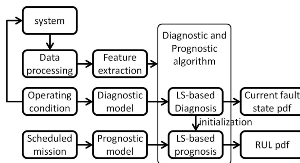
Figure 1. The implementation framework of LS-FDP
