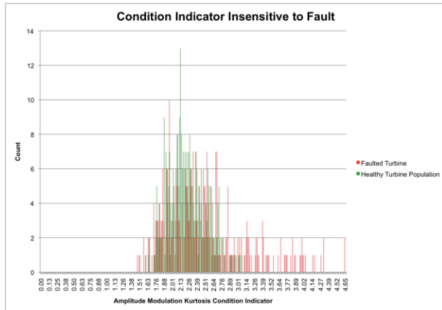
Figure 3. Fault discrimination based on AM Kurtosis
