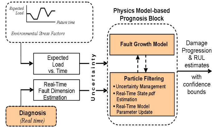
Figure 6. Model-based diagnostics and prognostics diagram.
