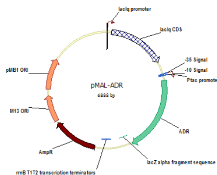
Figure 6: Vector pMAL-ADR containing human Adr.
