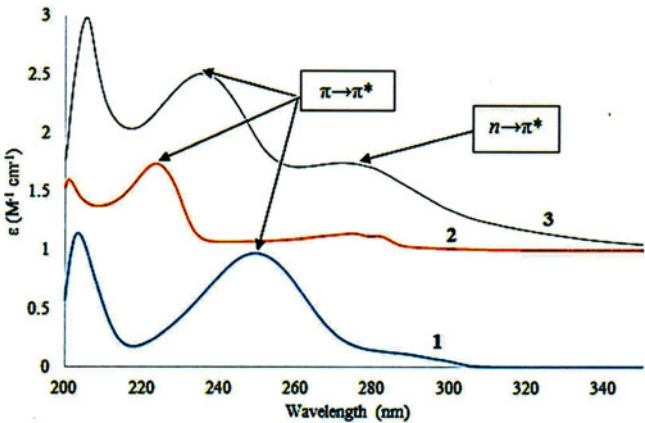
Figure 2. UV-Vis spectra for 1 , 2 and 3 .
