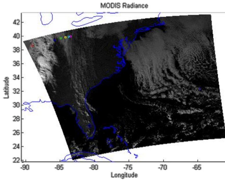
Figure 26. MODIS 1 km data granule. The seven squares in the northwest corner of the image correspond to the seven spectral radiance measurements plotted in Figure 27, providing a sample of several cloud-top heights and cloud types. Data collected 15 Dec 2014, 1815-1820 UTC.
