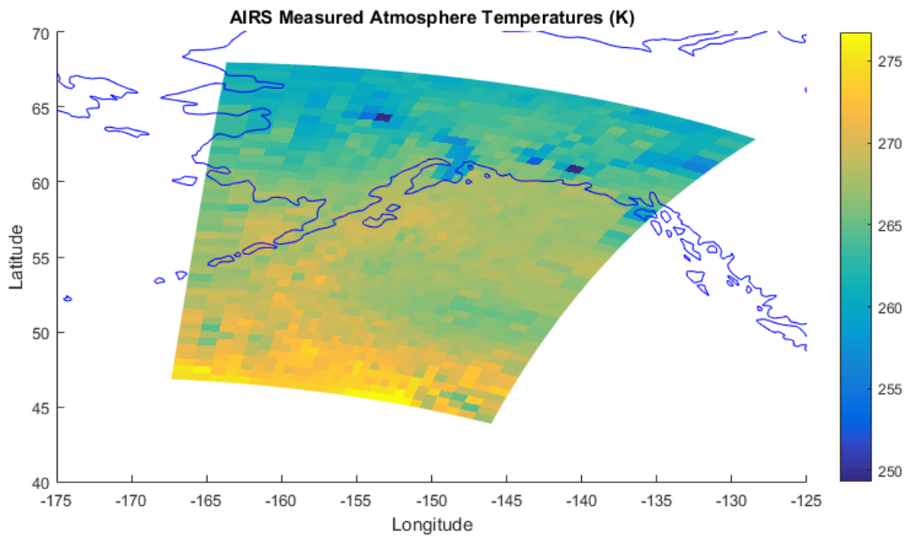
Figure 13. Horizontal slice through the volume of AIRS-retrieved temperatures contained in a 6-minute data granule at 753.6 hPa, 1229-1235 UTC, 15 Oct 2014.
