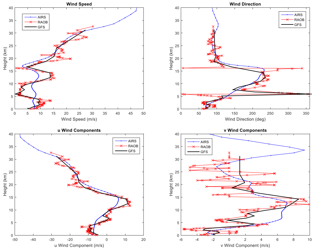
Figure 31. Comparison of AIRS-derived, RAOB-measured, and GFS-modeled wind profiles, Lihue, HI, 5 August, 2014, 0000 UTC.
