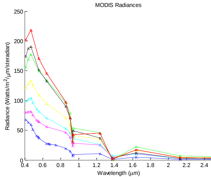
Figure 27. Calibrated MODIS radiance measurements. Each spectral radiance line corresponds to one of the MODIS fields-of-view identified in Figure 26.
