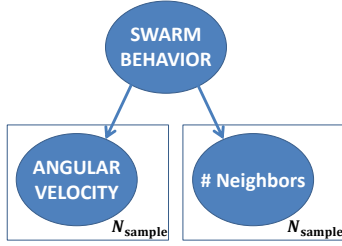
Figure 3: Bayesian network for swarm behavior classification using samples of local information from N_{\text{sample}} agents.
