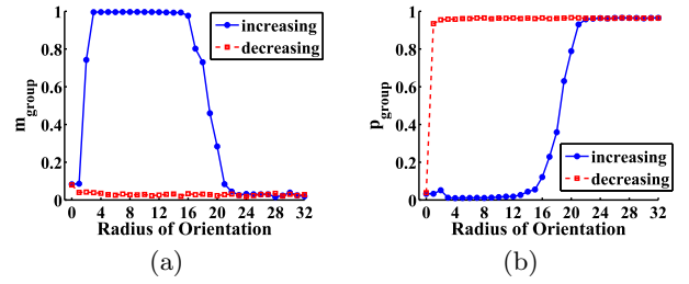
Figure 2: The average change in group momentum and polarization as the radius of orientation is increased and decreased.
