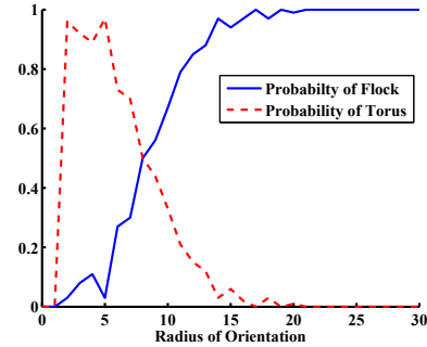
Figure 3: Probability of swarm forming a flock or a torus as a function of radius of orientation.
