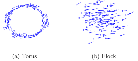
Figure 1: The two group types formed by our model. Agent headings are represented by straight lines.
