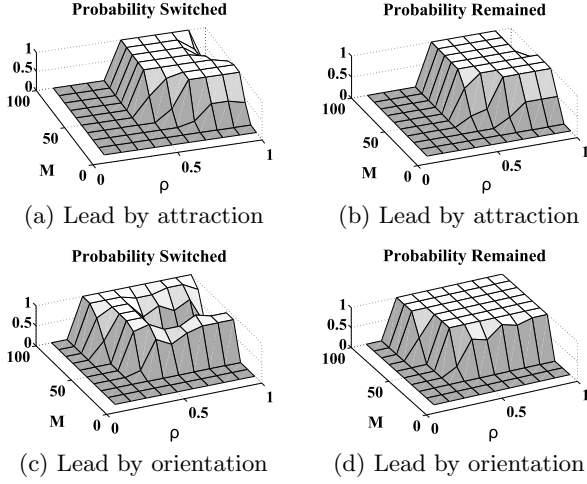
Figure 4: Switching from flock to torus.
