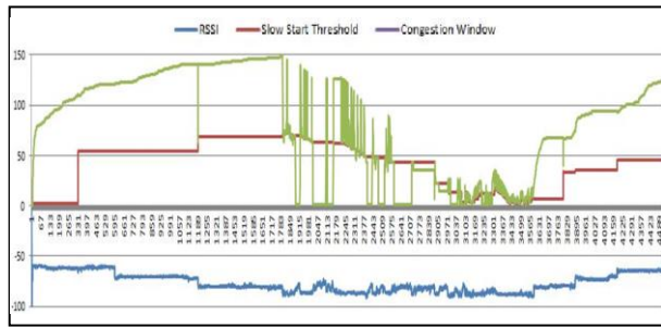
Figure 4: TCP Stockbridge congestion window size (packets) shown in Green, RSSI (dBm) is shown in blue, slow start threshold (packets) in shown in red.
