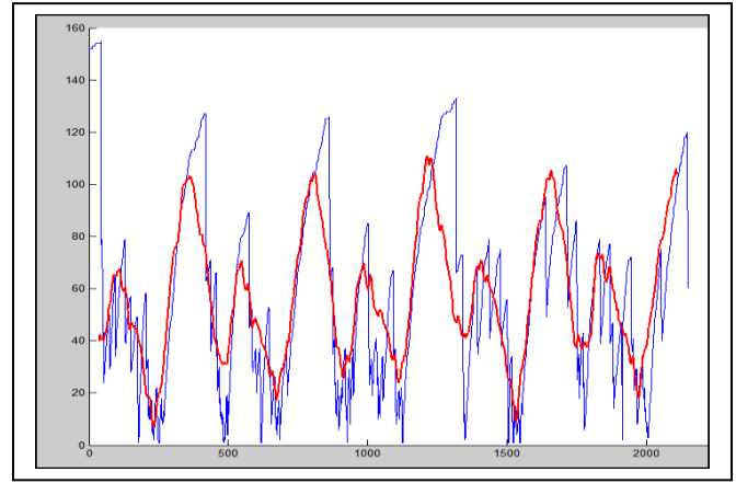
Figure 12: TCP Reno window size in Blue and SNR in Red
