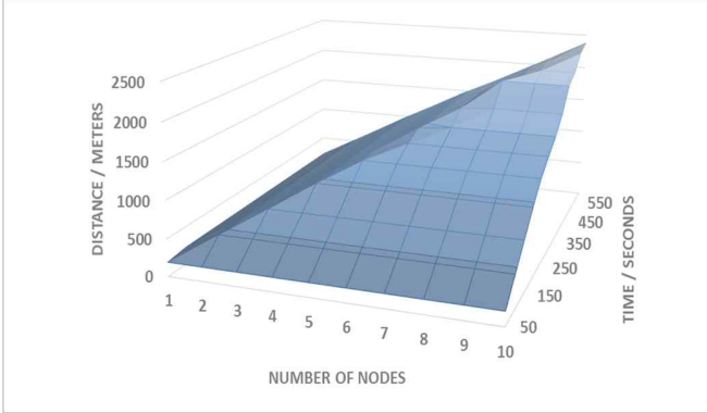
Figure 15: BioAIR scalability
