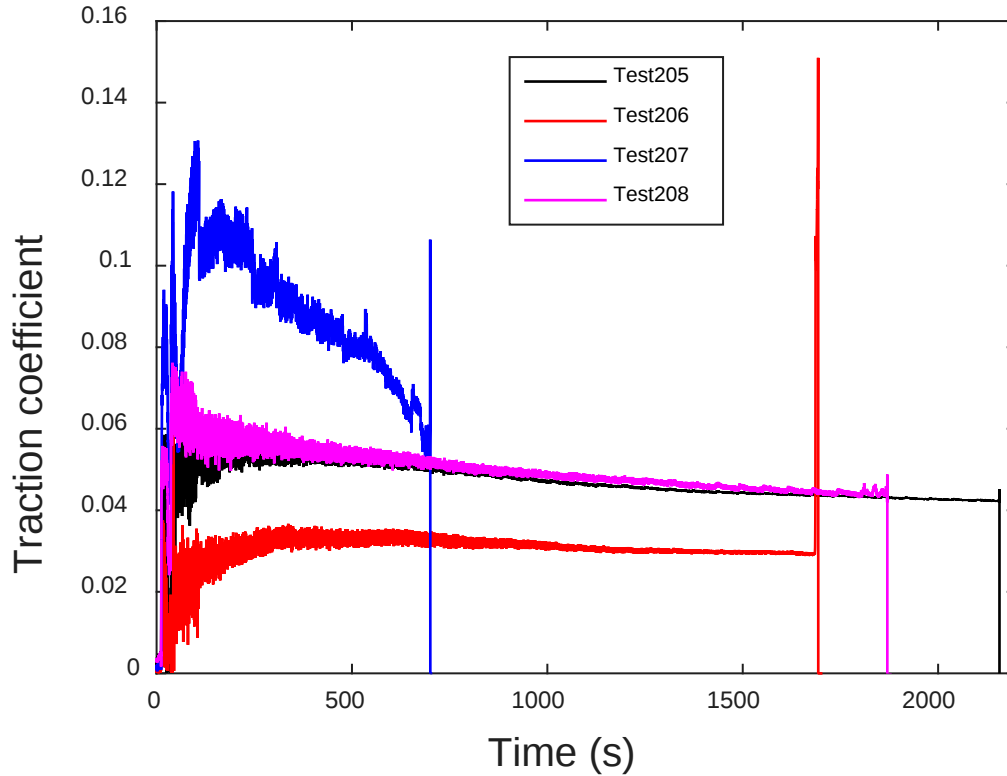
Fig. 11 LC traction-coefficient experimental data
