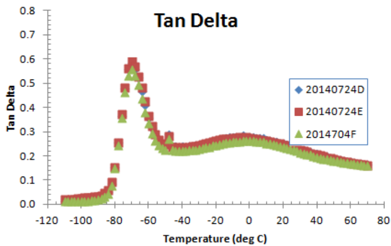
Figure 9 – DMA parameters for 1.0 Hz oscillations
