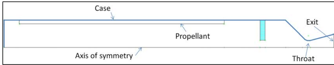
Figure 1: Motor components
