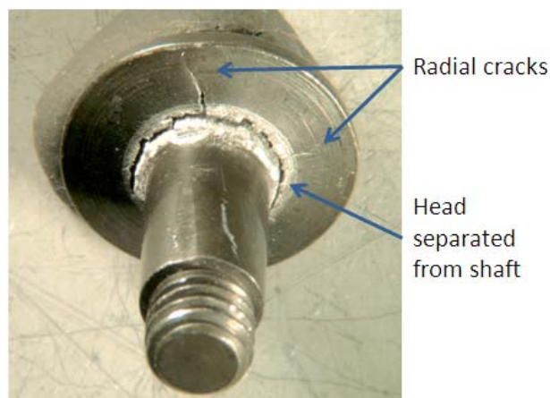
Figure 15. Example of severe damage inflicted by high force impact, showing circumferential cracking and radial cracking.
