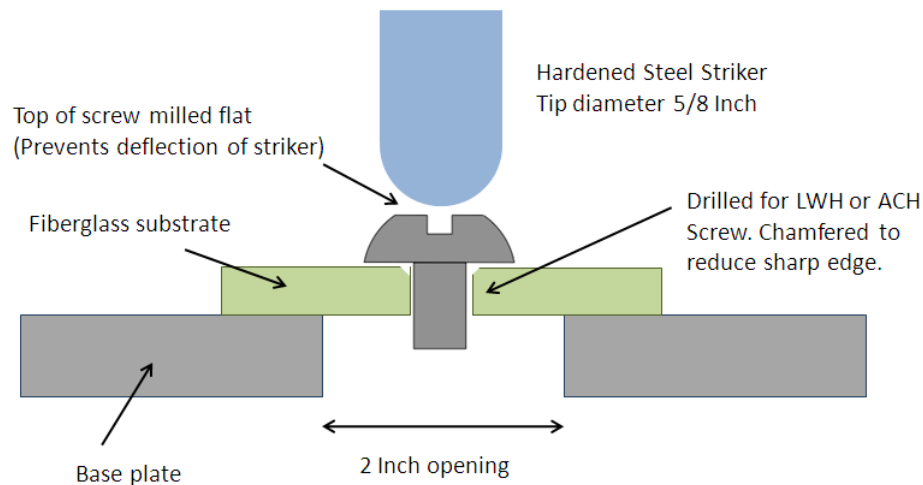
Figure 12. Schematic of the impact test configuration. The top of the screw was slightly flattened to prevent the rounded striker from deflecting. The substrate is \frac{1}{4} inch thick fiberglass plate supported on a base plate of 5083 aluminum alloy.
