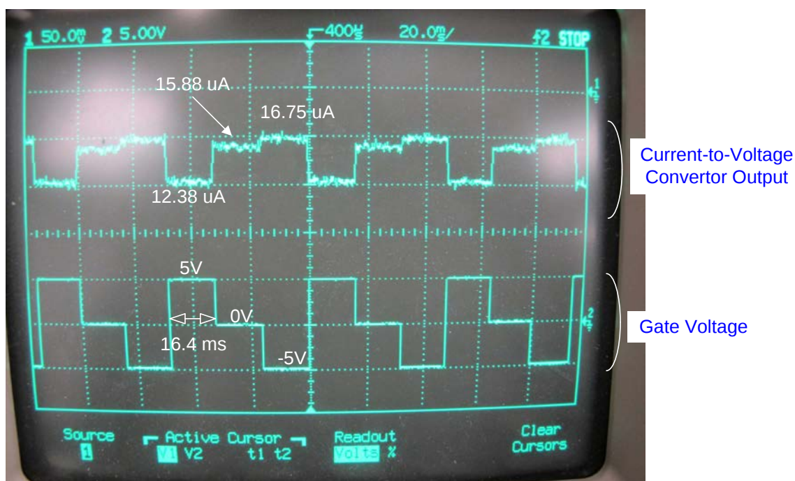
Figure 63 Oscilloscope Snapshot ( t_{\Delta V_{gate}} = 16.4 ms).
