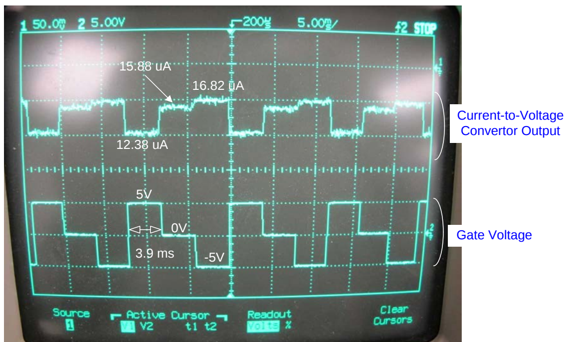
Figure 62 Oscilloscope Snapshot ( t_{\Delta V_{gate}} = 3.9 ms).
