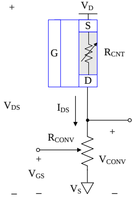
Figure 22 I-to-V Conversion (Resistor).
