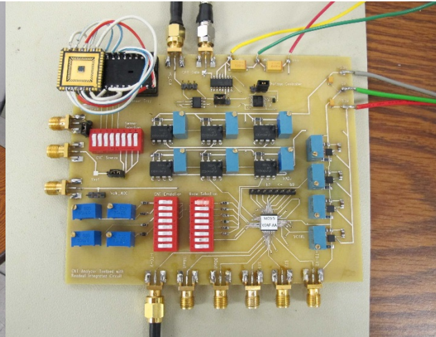
Figure 65 PCB Board Design.
