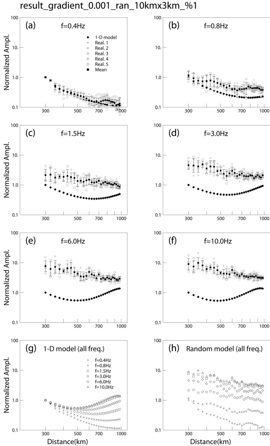
Figure 43. Pn wave spectral amplitude versus distance calculated from random velocity model Grad_0.001_ran_10kxm3km_1.0% (Model No 9 in Table 4). (a) to (f) are spectral amplitudes at 0.4, 0.8, 1.5, 3.0, 6 and 10 Hz. (g) Amplitudes in the 1D background model. Different symbols are for different frequencies. (h) Mean amplitudes for the random velocity model.
