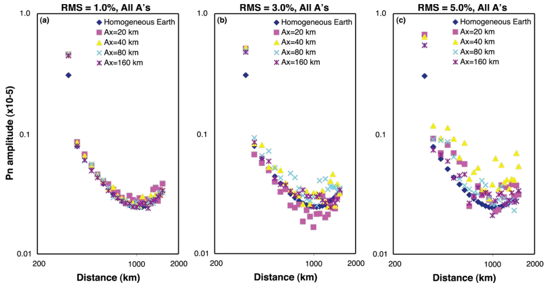
Figure 7. Ensemble-averaged \sim 1 -Hz P_n amplitudes plotted as a function of distance for all configurations of random Moho topography heterogeneity, grouped by percent RMS depth fluctuation. P_n amplitude for the BEM (diamonds) are compared to horizontal averaging length scales of 20 km (squares), 40 km (triangles), 80 km (X's), and 160 km (asterisks), for percent RMS depth fluctuations of (a) 1%; (b) 3%; and (c) 5%. From Avants et al. (2011).
