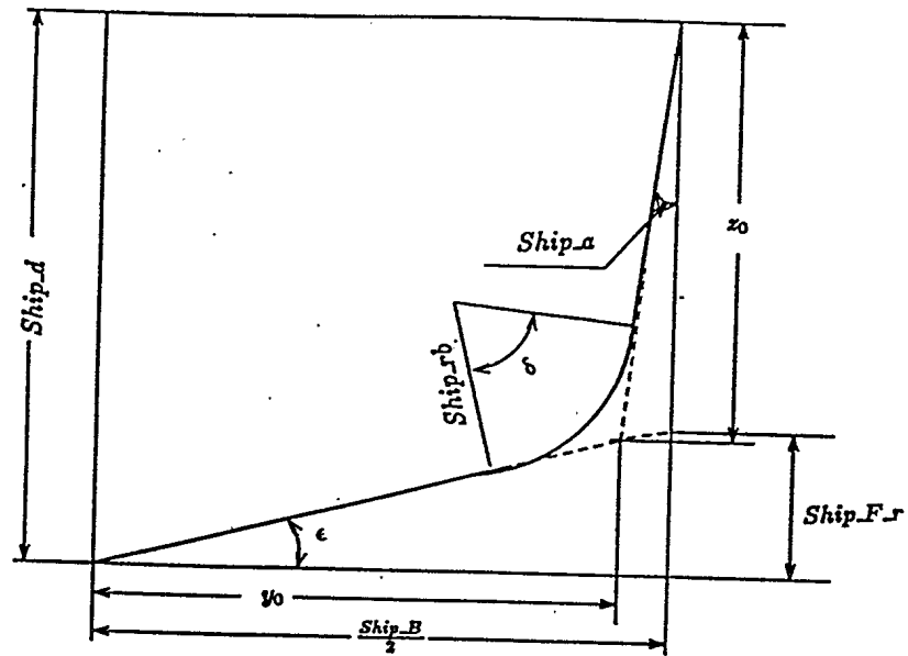
Figure 5: Sectional Parameters
