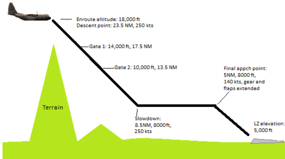
Figure 12: Sample Penetration Descent Profile
