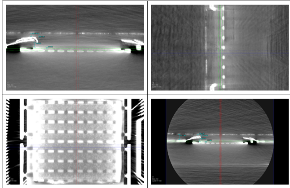
Figure 10 Xilinx Spartan-6 FPGA 3-D cross section X-Ray image taken by Steve Tetlak (AFRL/RD, 2015).
