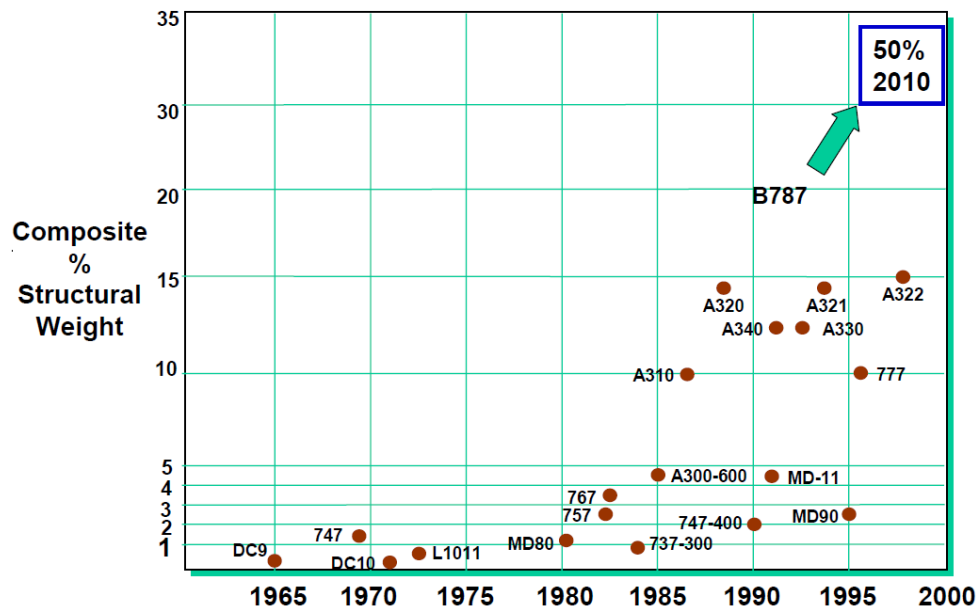
Figure 2. Composites Use in Commercial Transport Aircraft. Again, note the dramatic increase in the past 50 years. The Boeing 787 did indeed reach 50% composites by weight. Reproduced from [11].
