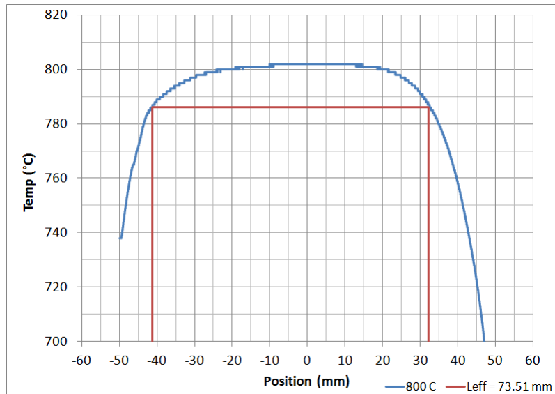
Figure A.12. Effective gauge length and temperature profile in silicic acid saturated steam for 800°C.
