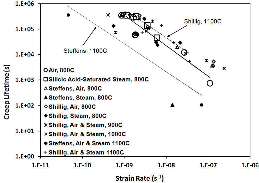
Figure 45. Monkman-Grant plot of creep lifetime vs. steady-state strain rate for Hi-Nicalon TM S SiC fiber tow specimens tested at 800°C in dry air, in steam, and in silicic acid-saturated steam with regression fits for 1100°C data. Data is from the current work and reproduced from Steffens [1] and Shillig [23]
