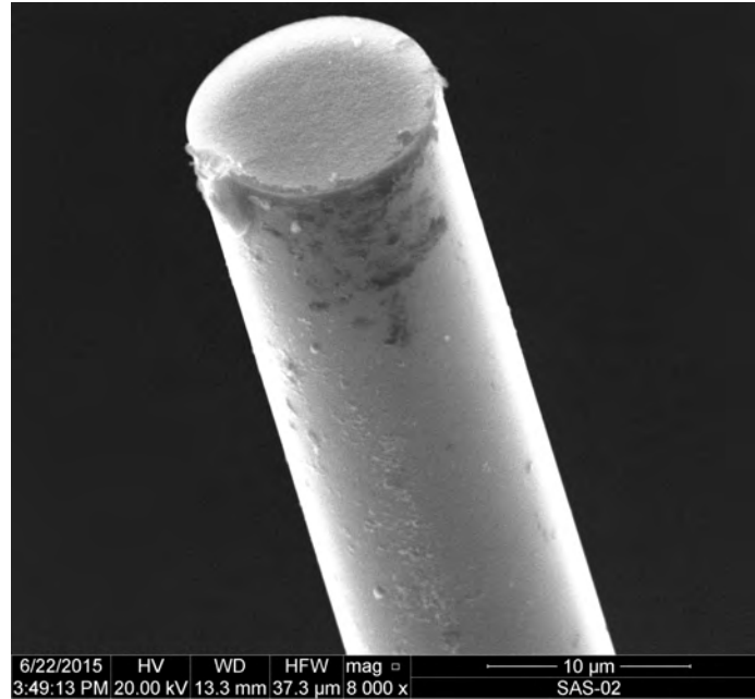
Figure 58. Brittle fracture of Hi-Nicalon TM S fiber tow specimens after creep rupture in silicic acid-saturated steam at 800°C.
