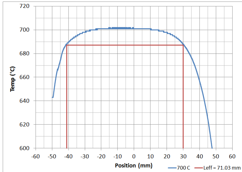
Figure A.11. Effective gauge length and temperature profile in silicic acid saturated steam for 700°C.
