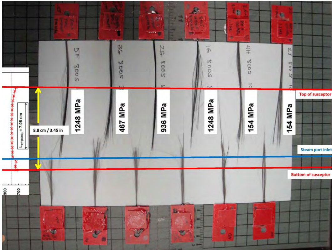
Figure 28. Effect of steam impinging on fiber tows upon entry into the test chamber, reproduced from [1]. Note that all specimens failed at the point of steam impingement.
