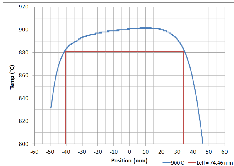
Figure A.6. Effective gauge length and temperature profile in Air for 900°C.
