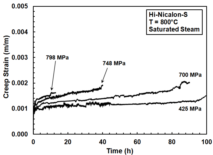
Figure 41. Representative creep curves for Hi-Nicalon TM S fibers at 800°C tested in silicic acid-saturated steam
