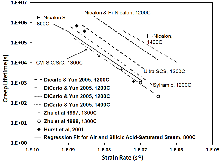
Figure 46. Monkman-Grant plot of creep lifetime vs. steady-state strain rate for Hi-Nicalon TM S SiC fiber tow specimens tested at 800°C in dry air and in silicic acid-saturated steam compared with data for various other SiC fibers and SiC/SiC CMCs. Data is from the current work and reproduced from DiCarlo et al [46], Zhu et al [191, 197], and Hurst et al [196]
