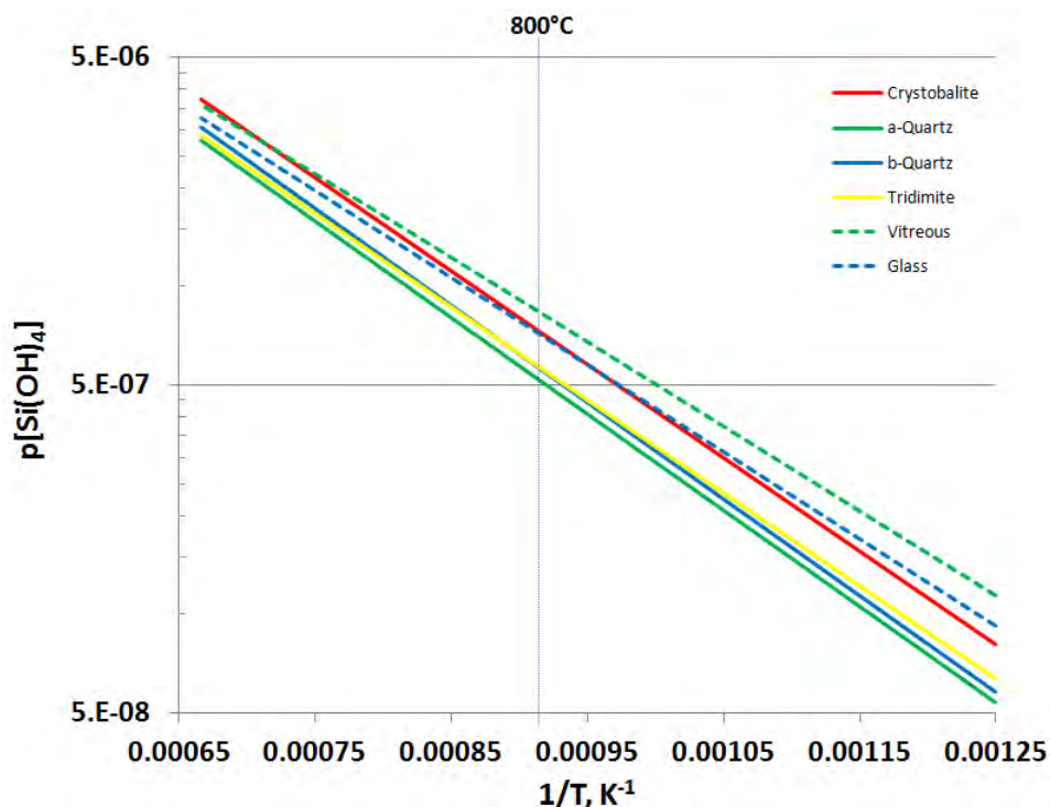
Figure 80. Equilibrium partial pressures of silicic acid in steam over various morphologies of silica. Data reproduced from [202] by Mogilevsky [203].
