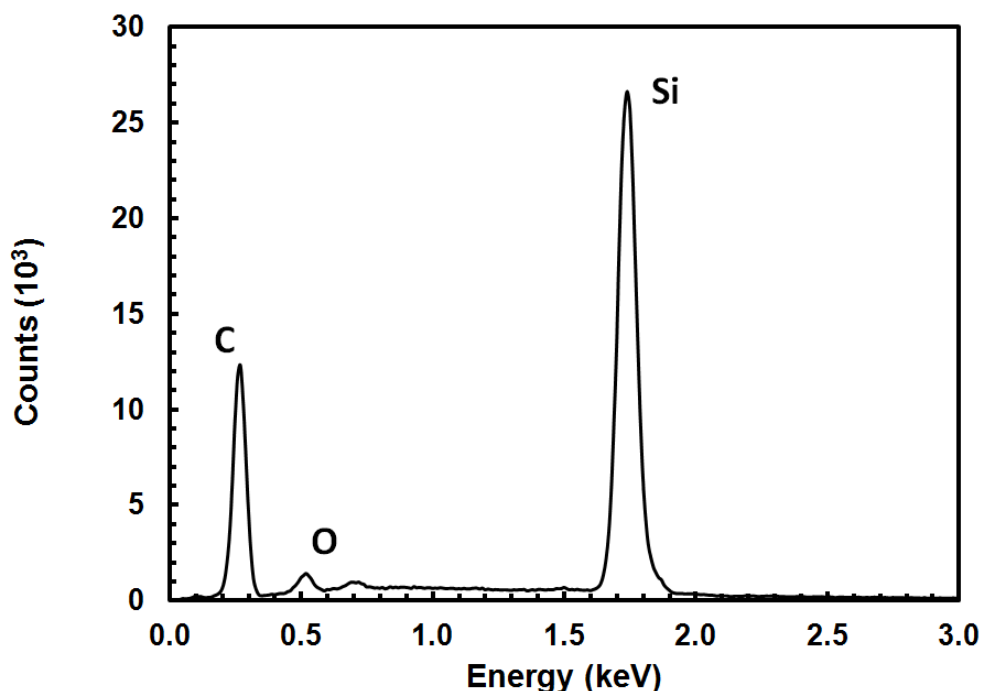
Figure 54. Energy dispersive spectrograph representative of the darker areas of the surface of Hi-Nicalon TM S SiC fiber tow specimen subjected to the saturated steam environment at 800°C and to a load of 2.96 MPa (429.3 psi). The composition is near stoichiometric SiC and a very small amount of oxygen. The content was 48.87% silicon, 49.09% carbon, and 1.51% oxygen by atomic percent.
