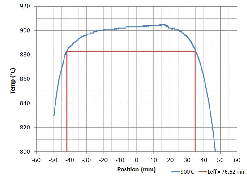
Figure A.13. Effective gauge length and temperature profile in silicic acid saturated steam for 900°C.
