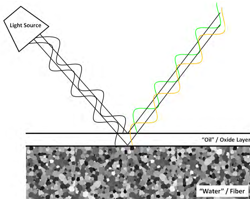
Figure 47. Schematic of constructive and destructive interference of light that causes interference fringes to be present during optical microscopy of oxidized fiber tows
