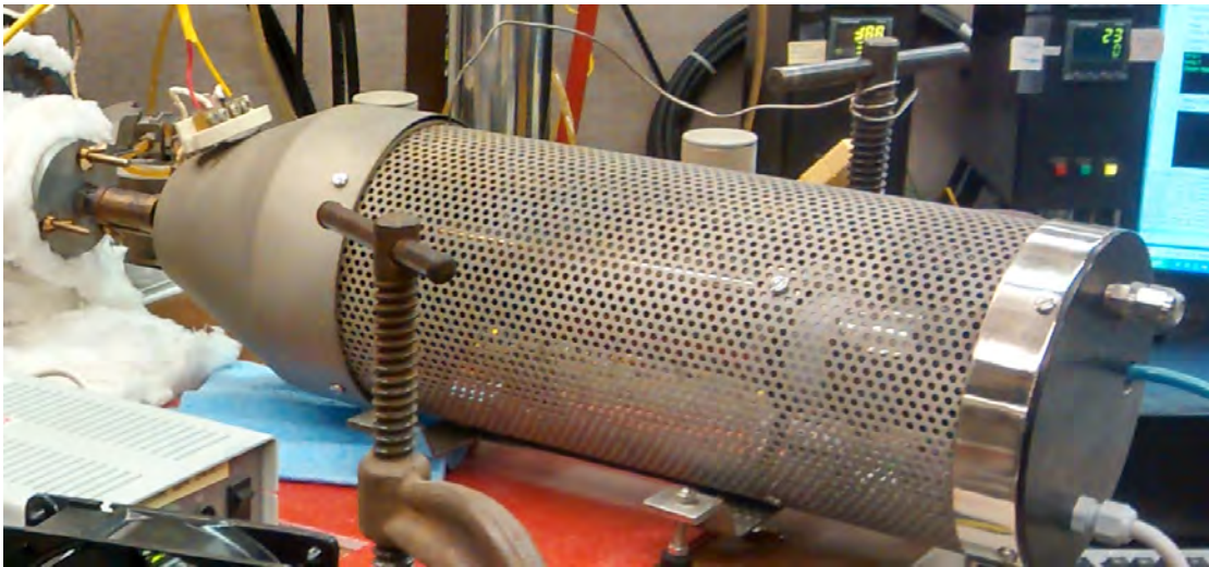
Figure 27. HGA-H (MHI) steam generator.
