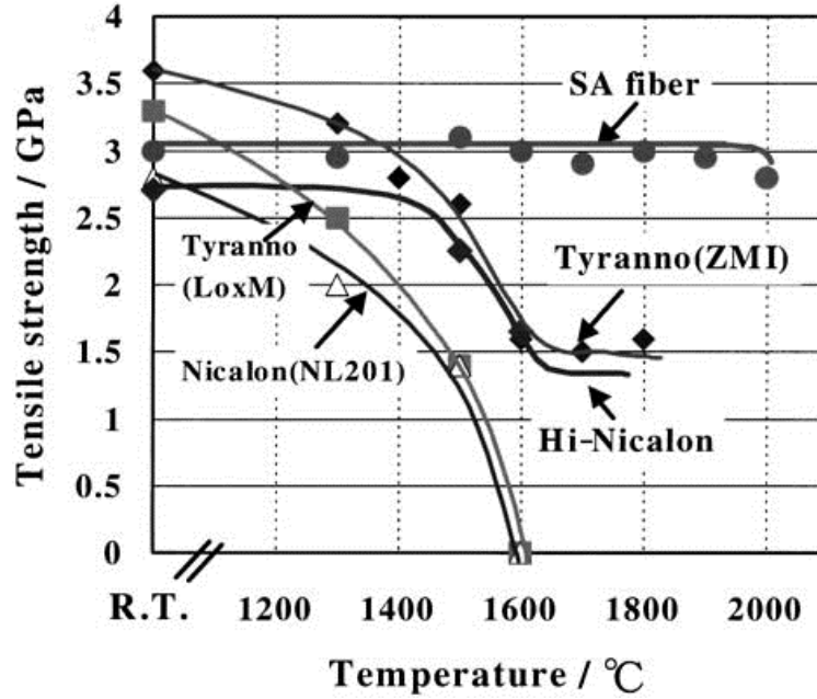
Figure 14. Temperature-dependent strength of third generation SiC fibers. Reproduced with kind permission from Springer Science & Business Media B.V. [20] pg. 121, Figure 14. Copyright ©2005 by Springer-Verlag Berlin Heidelberg.
