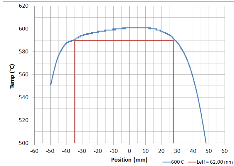
Figure A.3. Effective gauge length and temperature profile in Air for 600°C.
