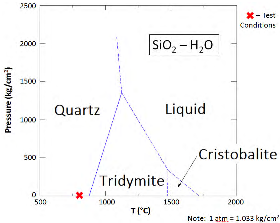
Figure 79. Phase Diagram for silica formation in a water environment. Note the red X depicting the test conditions during this research effort. Data reproduced from [201].
