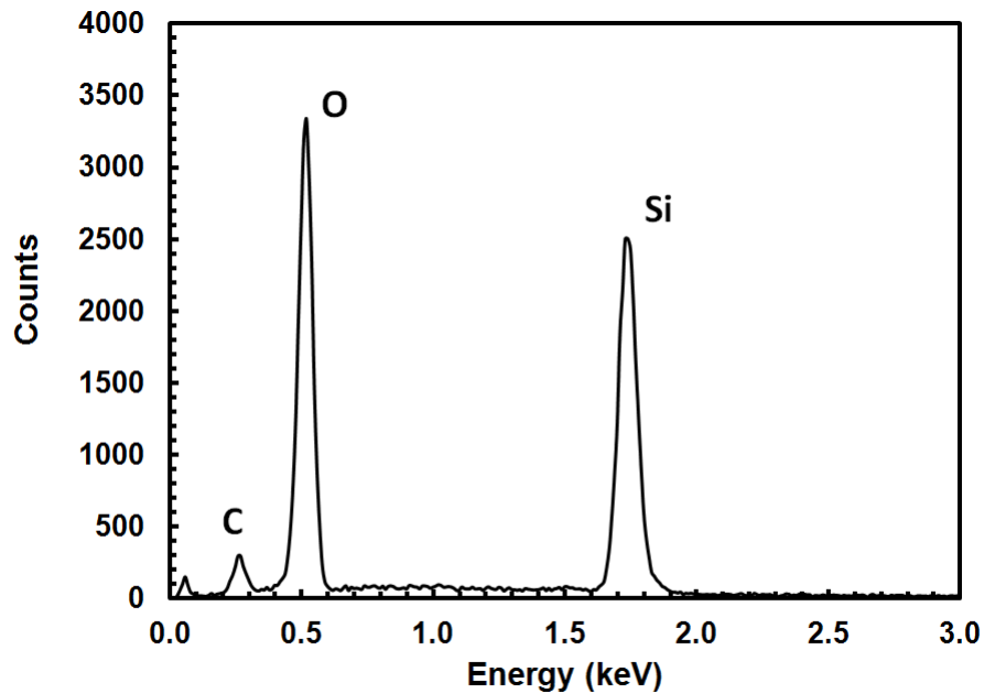
Figure 78. Energy dispersive spectrograph of the surface of “rogue” fiber from a Hi-Nicalon TM S SiC fiber tow specimen subjected to the saturated steam environment at 800°C and to a load of 450 MPa (65.3 ksi). The composition is representative of all EDS conducted on this morphology and is consistent with significant oxidation of the fiber to form a silica scale. The content was 42.86% silicon, 10.68% carbon, and 45.81% oxygen by atomic percent.
