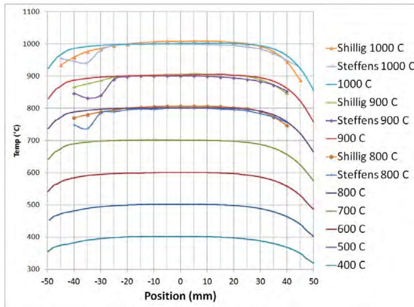
Figure 24. Temperature profiles in silicic acid saturated steam for the current work with data from Steffens [1] and Shillig [23] for comparison.
