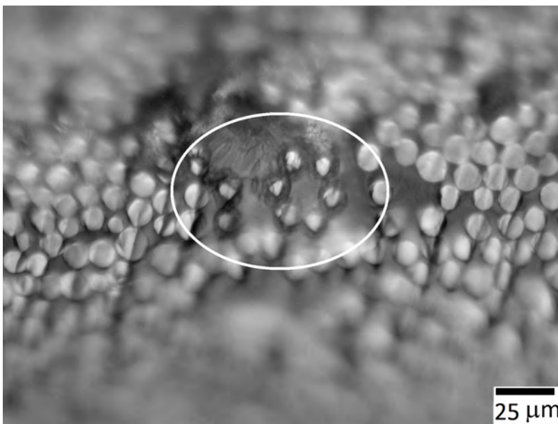
Figure 72. Optical micrograph of Hi-Nicalon TM S fiber tow specimens subjected to creep in silicic acid-saturated steam at 800°C and 625 MPa. Note the region in the center with a few fibers showing very large oxide scale.
