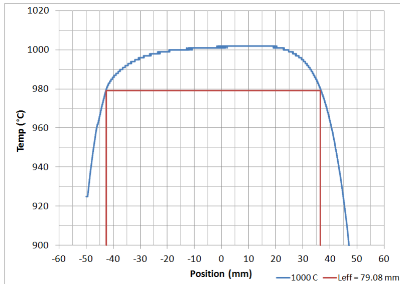
Figure A.14. Effective gauge length and temperature profile in silicic acid saturated steam for 1000°C.
