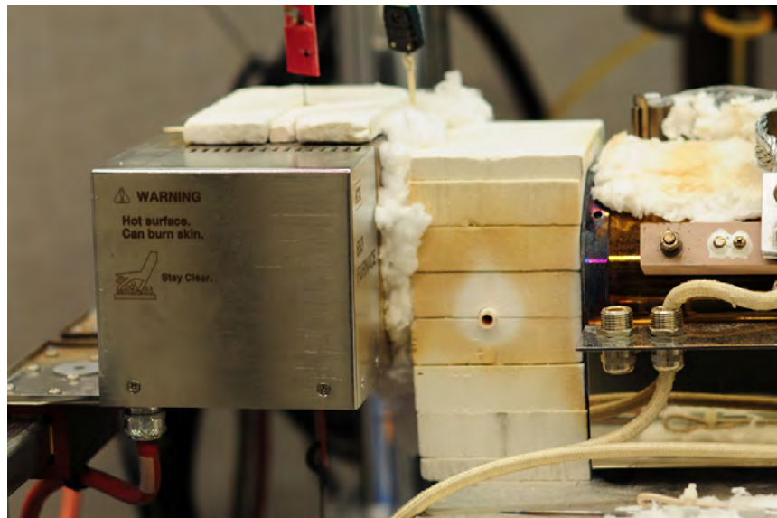
Figure 30. Layered insulation between CX1300 pre-heater and furnace, with steam bleed-off tube
