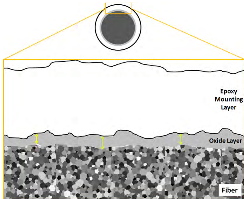
Figure 71. Schematic of a typical TEM image. Yellow arrows indicate multiple measurements taken and averaged to determine oxide thickness.
