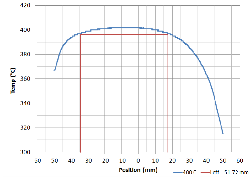
Figure A.1. Effective gauge length and temperature profile in Air for 400°C.
