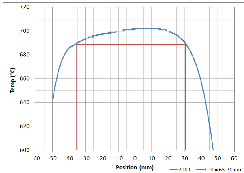
Figure A.4. Effective gauge length and temperature profile in Air for 700°C.
