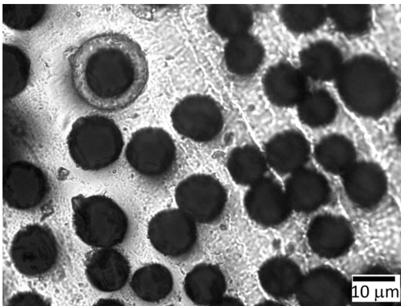
Figure 76. Optical micrograph of Hi-Nicalon TM S fiber tow specimen subjected to oxidation for 100 h at 700°C [198], used with permission.
