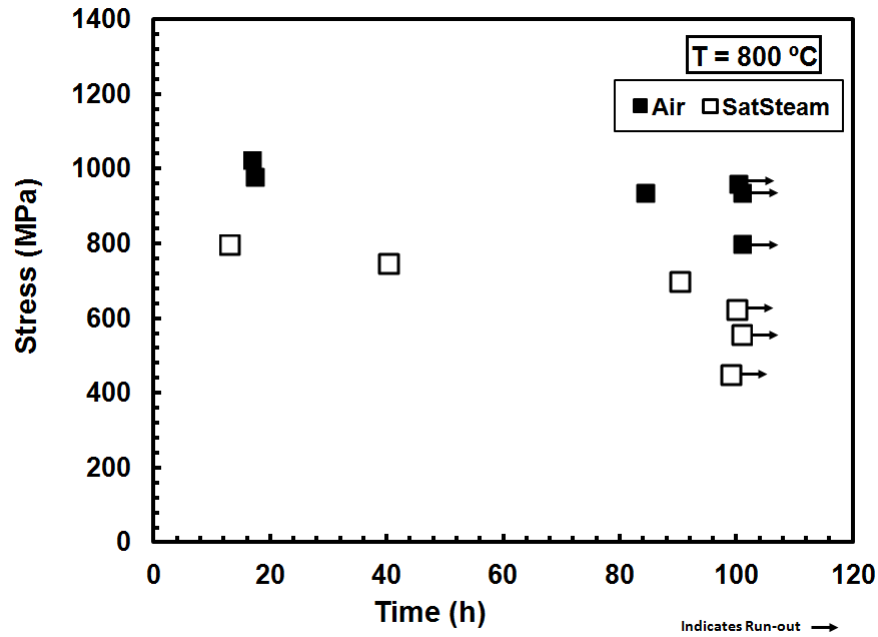
Figure 38. Creep Lifetimes of Hi-Nicalon TM S fibers at 800°C in air and in steam
