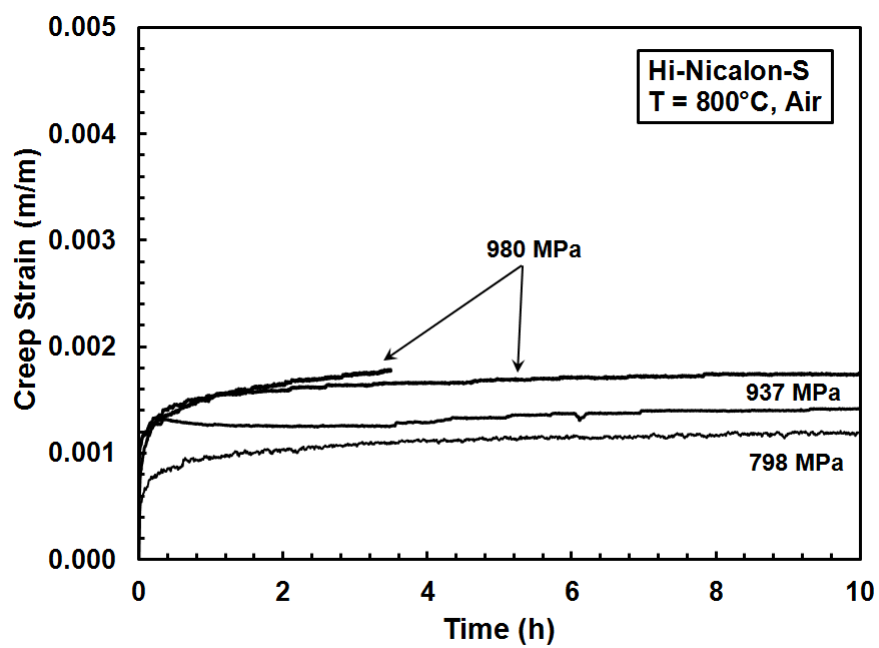
Figure 40. Representative creep curves for early stages of creep of Hi-Nicalon TM S fibers at 800°C in air
