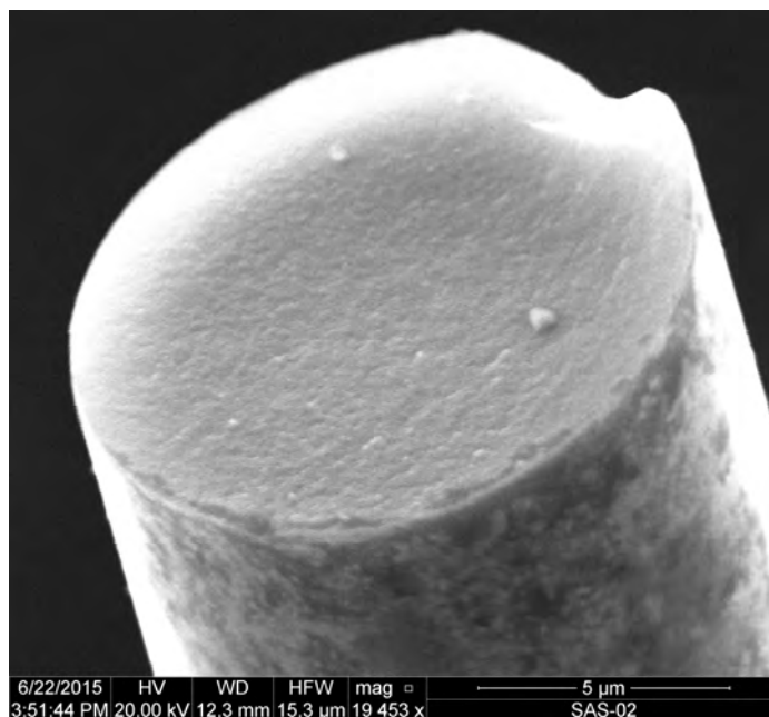
Figure 62. Rough, dark areas seen around fractures of Hi-Nicalon TM S fiber tow specimens subjected to creep in silicic acid-saturated steam at 800°C are likely the crack initiation sites.
