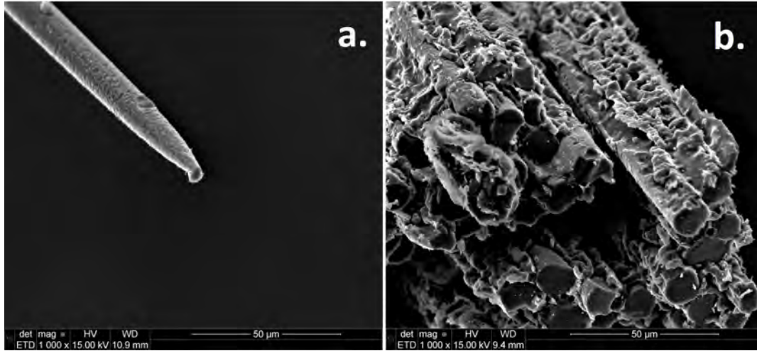
Figure 48. Variations along the fiber tow due to testing in unsaturated steam. a.) Fiber degradation due to active oxidation, typically found in sections of the fiber tow near the bottom of the test chamber. b.) Silica (SiO 2 ) scale growth typically found in sections of the fiber tow near the top of the test chamber. Reproduced from [23]
