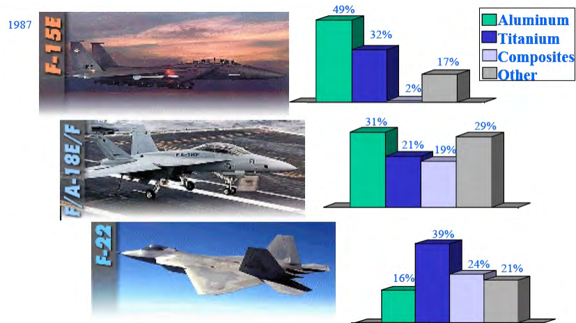
Figure 1. Composites Use in Military Aircraft. Note the dramatic increase in just 30 years. Reproduced from [11].
