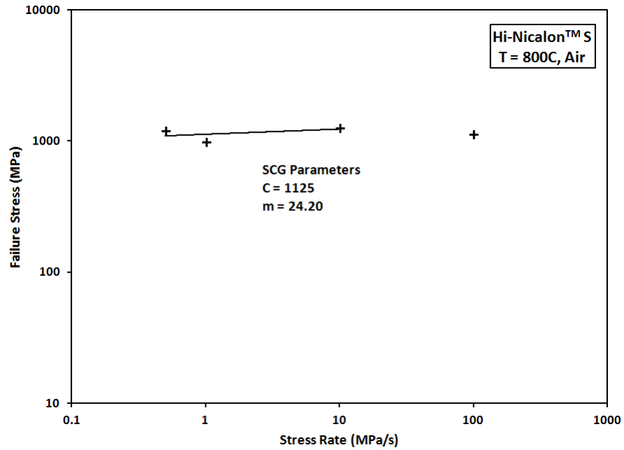
Figure 35. Failure Stress of Hi-Nicalon TM S fibers at 800°C in air as a function of stress rate. The effect of loading rate is minimal.
