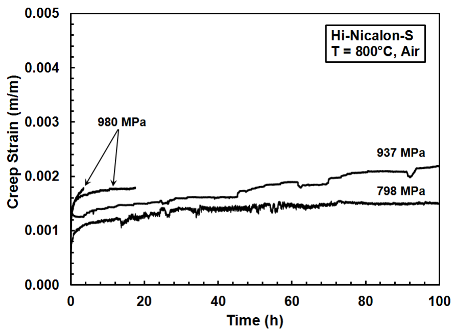
Figure 39. Representative creep curves for Hi-Nicalon TM S fibers at 800°C in air
