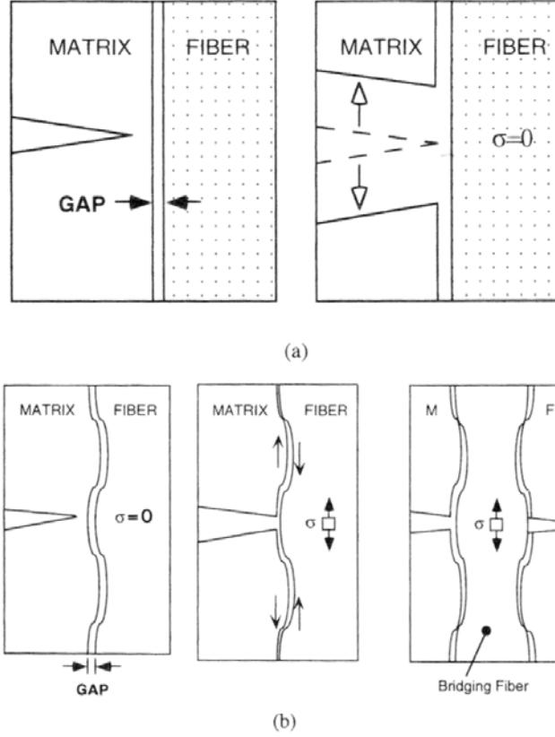
Figure 9. Load Transfer at Fiber/Matrix Interfaces with a Fugitive Coating: a) An idealized (smooth) interface would protect the fiber from the matrix crack, but no load transfer would occur, whereas b) in reality, the interface is rough and load transfer occurs while still protecting the fiber [39], reproduced with permission from Wiley.
