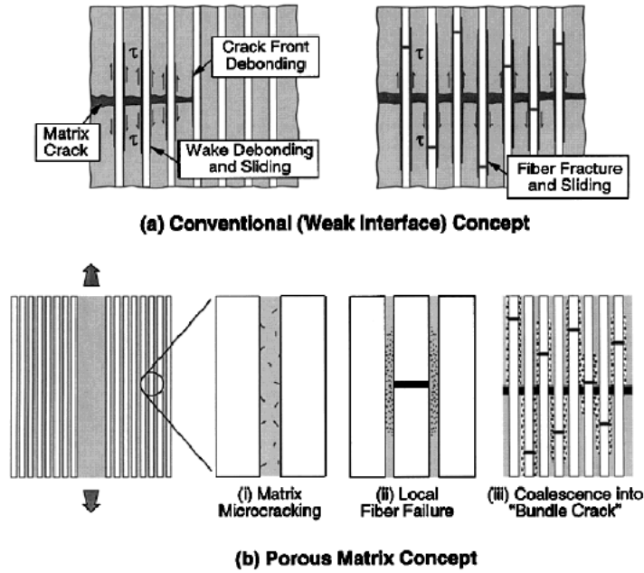
Figure 6. Design Methods for Damage Tolerant CMCs: a) fiber coating with weak fiber/matrix interface and b) porous matrix [16], reproduced with permission from Wiley.
