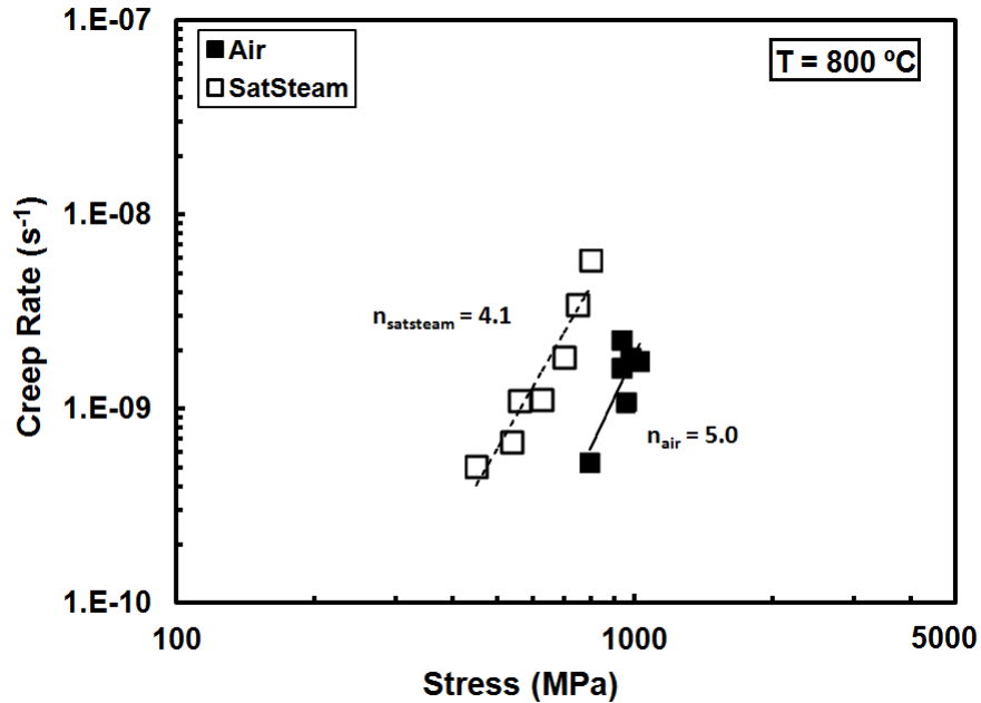
Figure 37. Creep strain rate vs. applied stress for Hi-Nicalon TM S fibers tows at 800°C in air and in steam, with associated creep exponents
