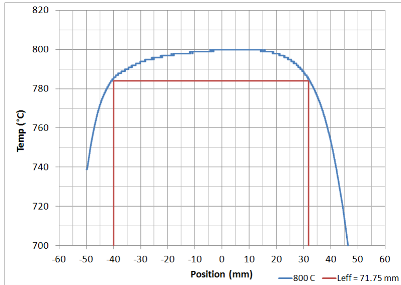
Figure A.5. Effective gauge length and temperature profile in Air for 800°C.
