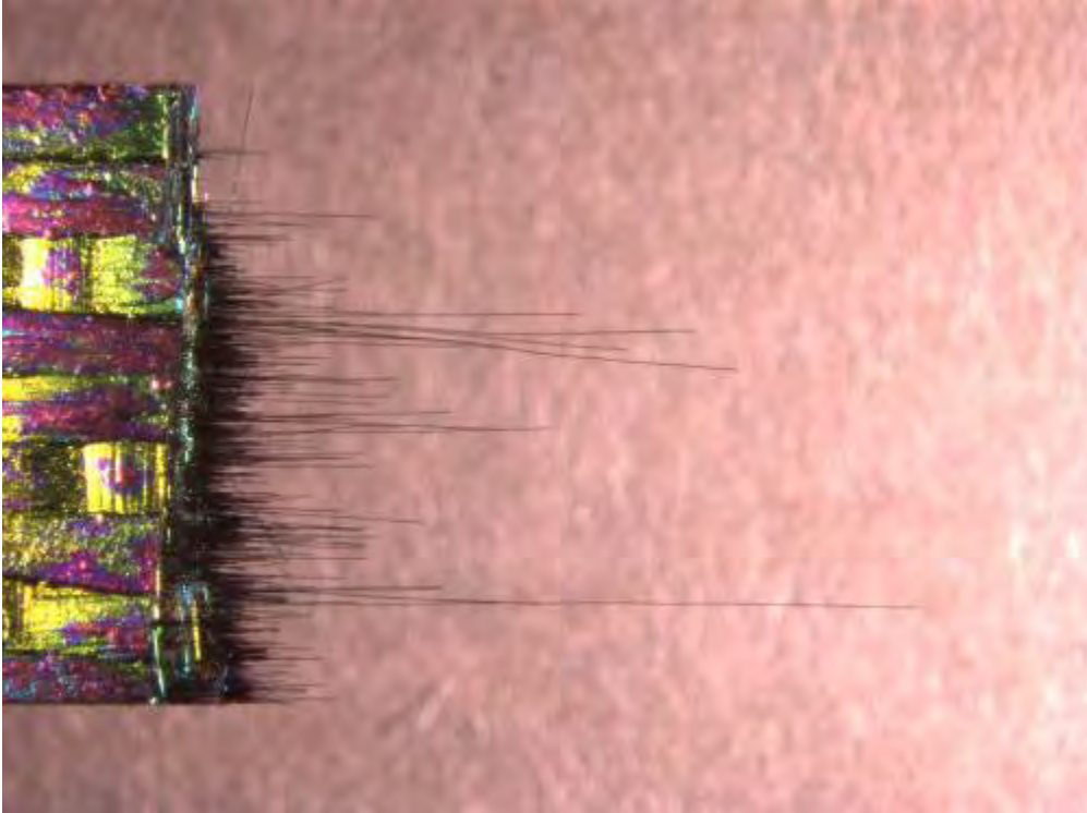
Figure 7. Fiber pullout in SiC/BN/SiC CMC after a tensile fatigue test at 1200°C in air. Note the substantial amount of fiber pullout. Reproduced from [30].
