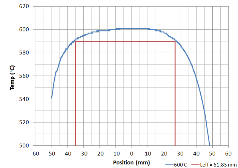
Figure A.10. Effective gauge length and temperature profile in silicic acid saturated steam for 600°C.
