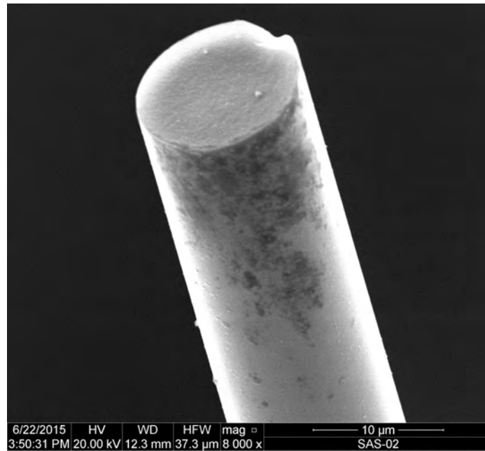
Figure 61. Rough, dark areas seen around fractures of Hi-Nicalon TM S fiber tow specimens subjected to creep in silicic acid-saturated steam at 800°C are likely the crack initiation sites.
