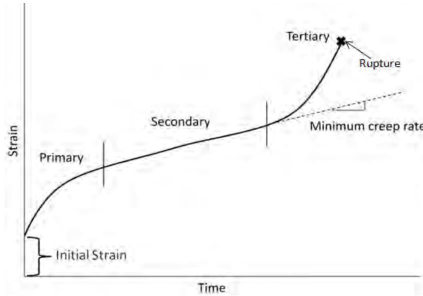
Figure 16. Phases of a typical creep curve. Reproduced from [4], with initial strain and rupture notations added.
