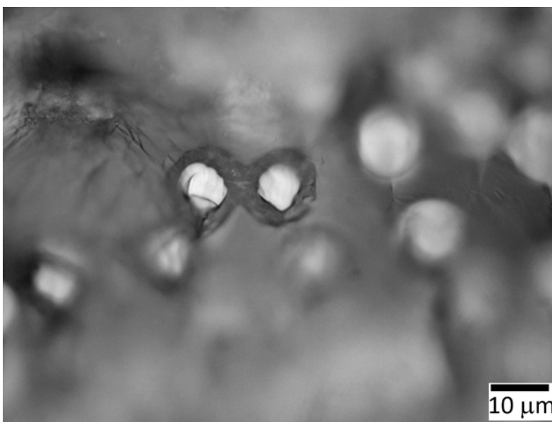
Figure 73. Optical micrograph of Hi-Nicalon TM S fiber tow specimens subjected to creep in silicic acid-saturated steam at 800°C and 625 MPa.
