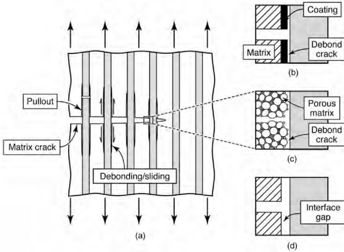
Figure 8. Current Design Philosophies for Damage Tolerant CMCs: a) damage tolerant design concept showing uncorrelated fiber failure, debonding, and pullout b) fiber coating with weak fiber/matrix interface, c) porous matrix, and d) fugitive coating [29], reproduced with permission from Wiley.
