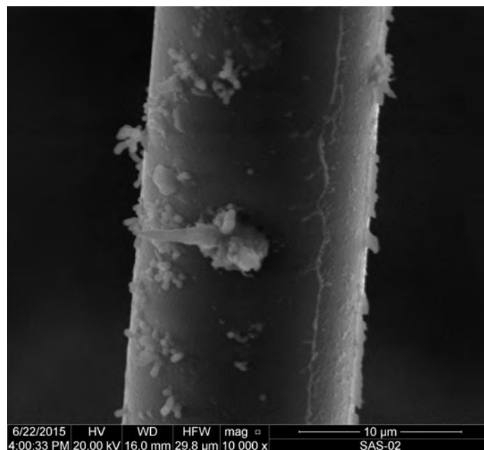
Figure 64. Crystalline deposits of silica likely precipitated out of the silicic acid-saturated steam environment during creep tests of Hi-Nicalon TM S fiber tow specimens at 800°C.
