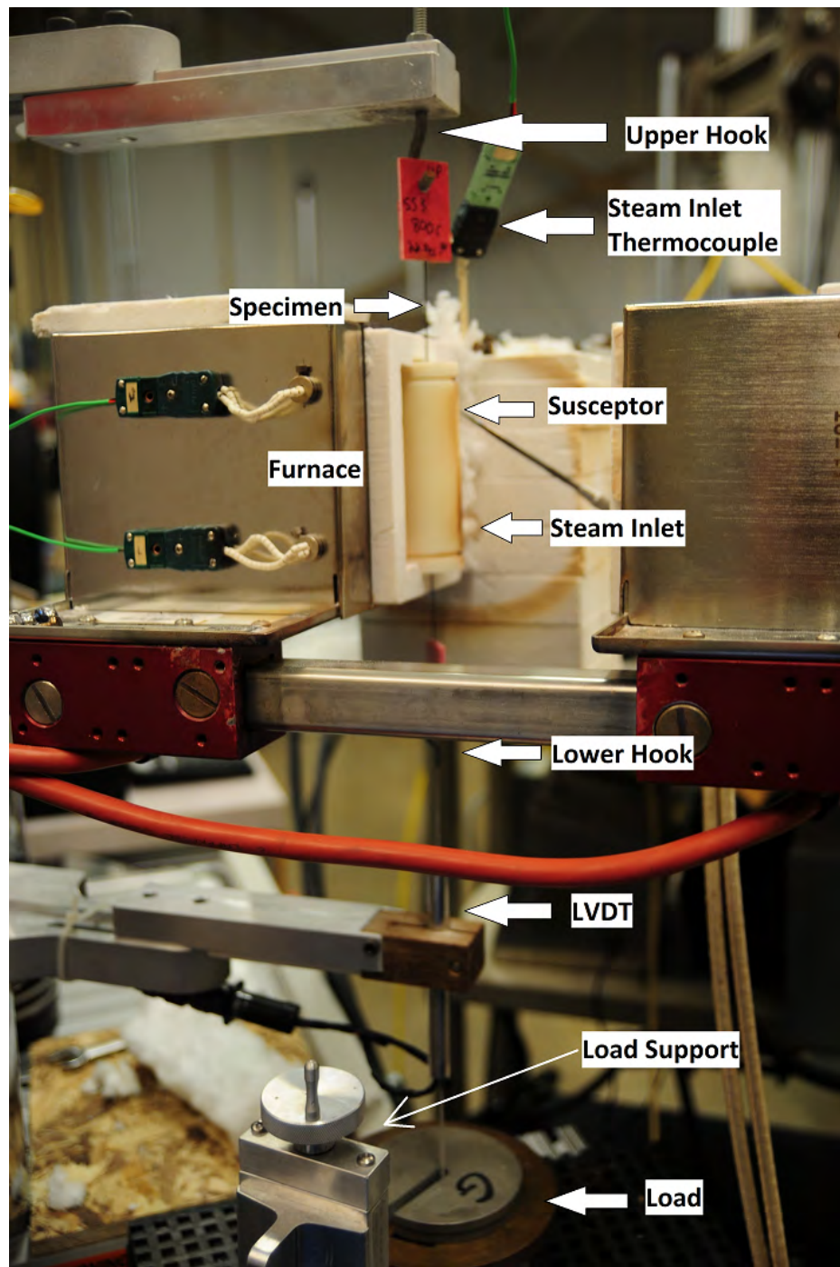
Figure 22. Fiber tow creep test setup
