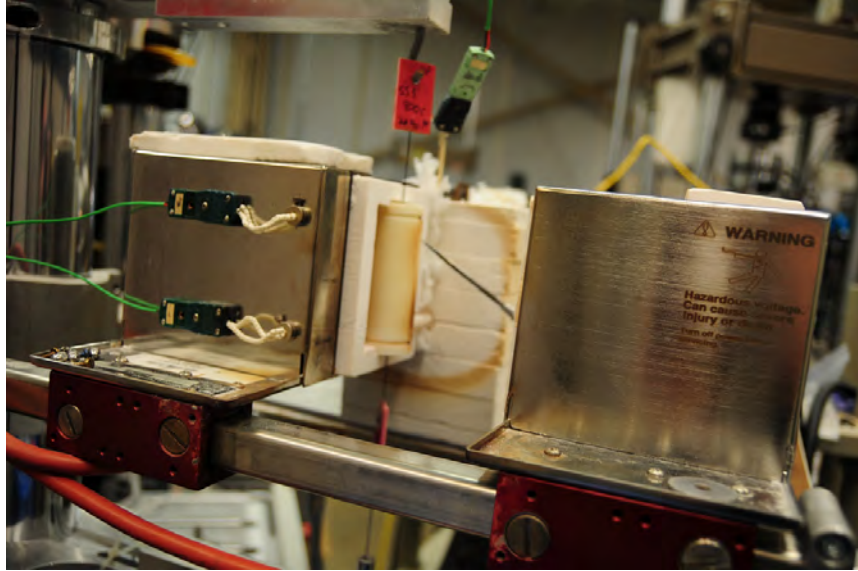
Figure 20. Two-zone resistance-heated MTS 653.03A furnace with silicon carbide heating elements, R type control thermocouples and a 90 mm (3.5 in.) hot zone
