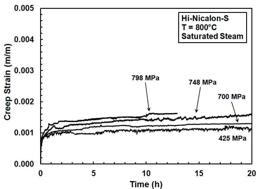
Figure 42. Representative creep curves for early stages of creep of Hi-Nicalon TM S fibers at 800°C tested in silicic acid-saturated steam
