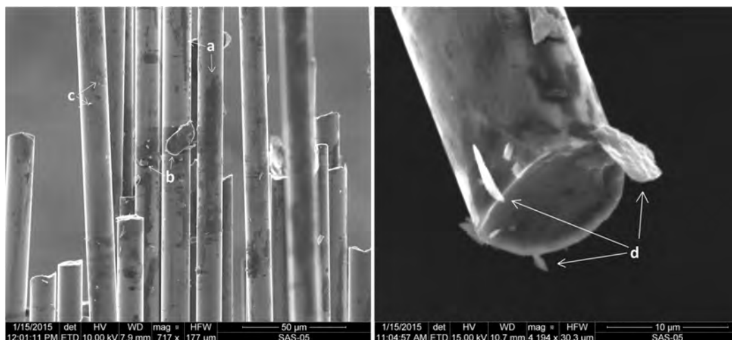
Figure 55. Common surface features of Hi-Nicalon TM S SiC fiber tow specimens subjected to the saturated steam environment at 800°C and to a load of 2.96 MPa (429.3 psi). Note the a) smooth, mottled surface, b) large chunks of fiber, c) small precipitates of silica, and d) small flakes of the silica oxide layer.
