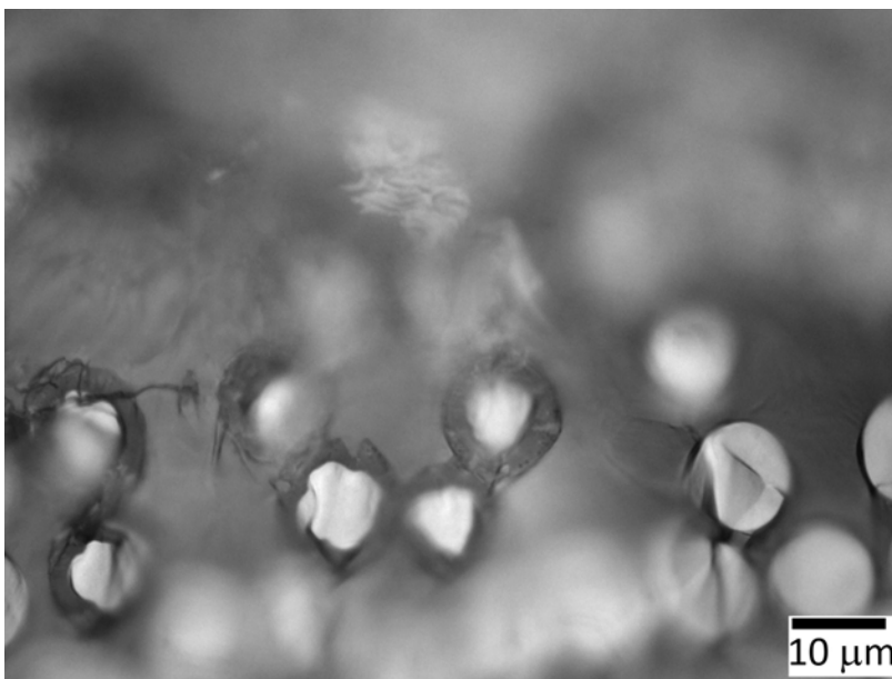
Figure 74. Optical micrograph of Hi-Nicalon TM S fiber tow specimens subjected to creep in silicic acid-saturated steam at 800°C and 625 MPa.
