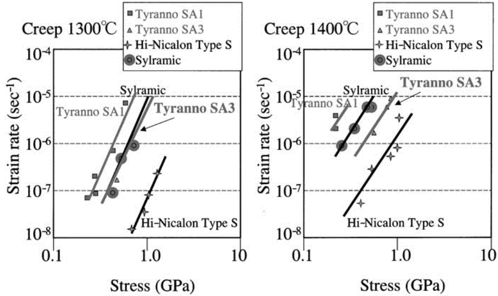
Figure 15. Creep of third generation SiC fibers. Reproduced with kind permission from Springer Science & Business Media B.V. [20] pg. 122, Figure 15. Copyright ©2005 by Springer-Verlag Berlin Heidelberg.
