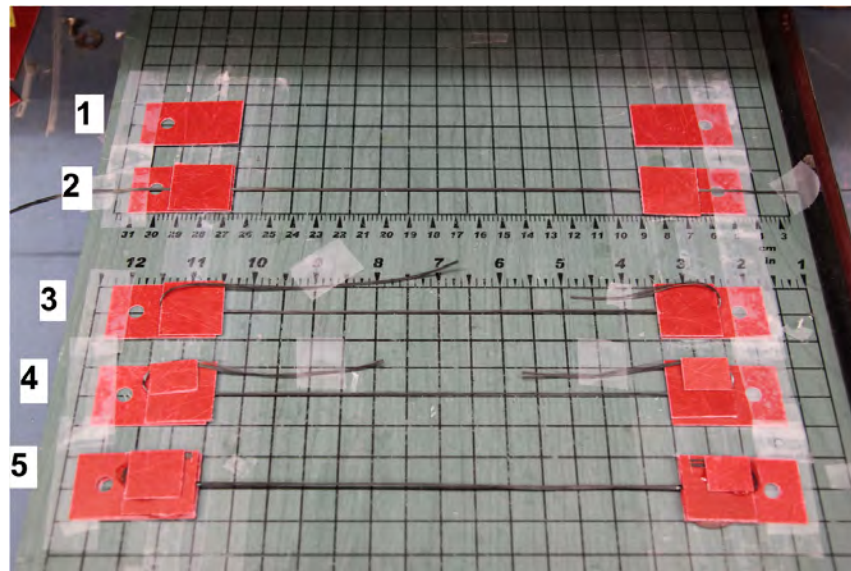
Figure 26. Fiber tow creep test specimen preparation process, reproduced from [23]
