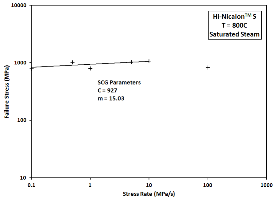
Figure 36. Failure Stress of Hi-Nicalon TM S fibers at 800°C in silicic acid-saturated steam as a function of stress rate. The effect of loading rate is minimal.
