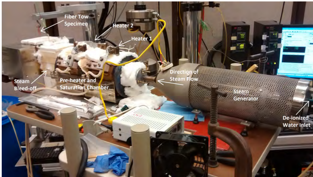
Figure 31. Saturated steam creep test facility
