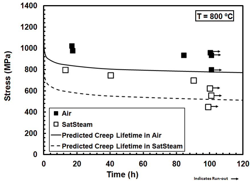
Figure 43. Model predictions of creep lifetime compared to actual creep lifetime data for Hi-Nicalon TM S SiC fiber tow specimens tested at 800°C in dry air and in silicic acid-saturated steam.
