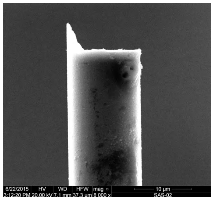
Figure 67. Contaminants introduced during fabrication, preparation, or testing of Hi-Nicalon TM S fiber tow specimens subjected to creep in silicic acid-saturated steam at 800°C can cause increased localized oxidation, often resulting in failure of the fiber at or near the location of the contaminant.
