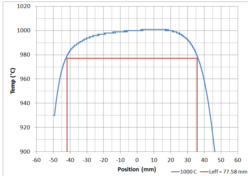
Figure A.7. Effective gauge length and temperature profile in Air for 1000°C.
