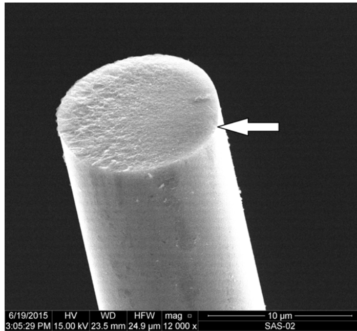
Figure 57. Brittle fracture of Hi-Nicalon TM S fiber tow specimens after creep rupture in air at 800°C.
