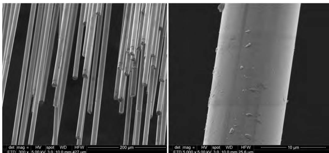
Figure 50. Center section of Hi-Nicalon TM S SiC fiber tow specimen subjected to the saturated steam environment at 800°C and to a load of 2.96 MPa (429.3 psi)
