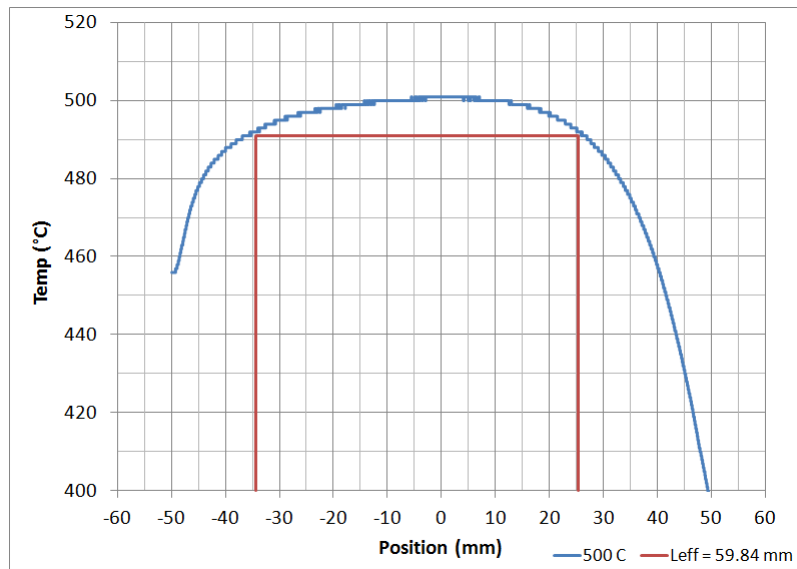
Figure A.2. Effective gauge length and temperature profile in Air for 500°C.
