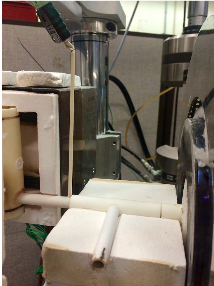
Figure 29. Bleed-off assembly between CX1300 pre-heater and test chamber inside the furnace, with steam inlet thermocouple
