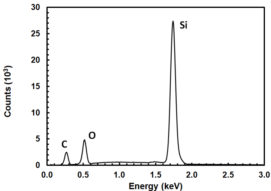
Figure 52. Energy dispersive spectrograph representative of the lighter areas of the surface of Hi-Nicalon TM S SiC fiber tow specimen subjected to the saturated steam environment at 800°C and to a load of 2.96 MPa (429.3 psi). The composition shows an increase in silicon content from stoichiometric SiC, an accompanying decrease in carbon, and some oxygen. The content was 72.96% silicon, 16.29% carbon, and 9.72% oxygen by atomic percent.
