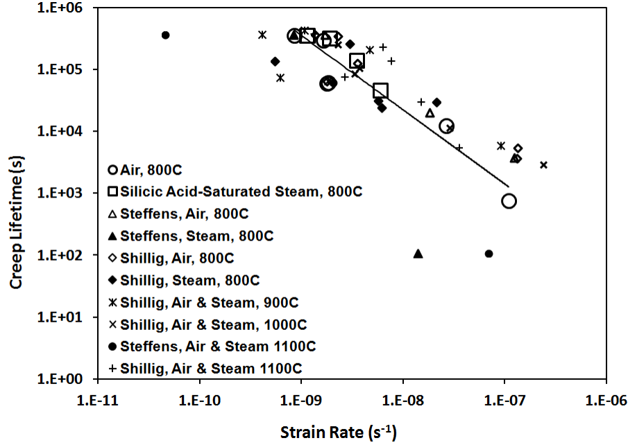
Figure 44. Monkman-Grant plot of creep lifetime vs. steady-state strain rate for Hi-Nicalon TM S SiC fiber tow specimens tested at 800°C in dry air, in steam, and in silicic acid-saturated steam. Data is from the current work and reproduced from Steffens [1] and Shillig [23]
