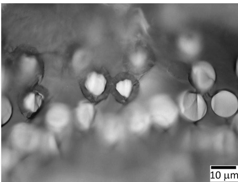
Figure 75. Optical micrograph of Hi-Nicalon TM S fiber tow specimens subjected to creep in silicic acid-saturated steam at 800°C and 625 MPa.
