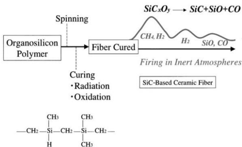
Figure 13. Production process for Hi-Nicalon TM S SiC fibers by electron irradiation curing and pyrolysis. Reproduced with kind permission from Springer Science & Business Media B.V. [20] pg. 117, Figure 8. Copyright ©2005 by Springer-Verlag Berlin Heidelberg.
