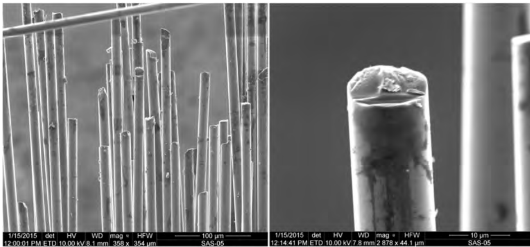
Figure 49. Lower section of Hi-Nicalon TM S SiC fiber tow specimen subjected to the saturated steam environment at 800°C and to a load of 2.96 MPa (429.3 psi)
