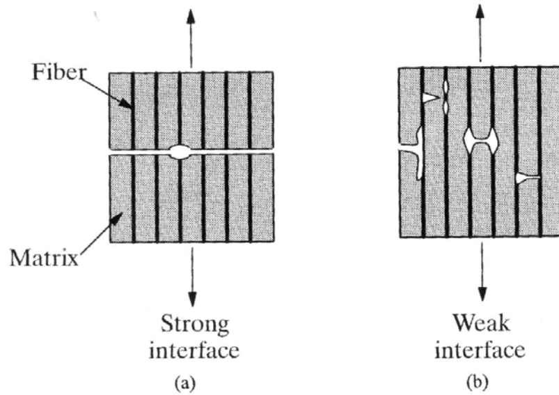
Figure 5. Failure of CFCCs showing crack propagation for strong and weak interface bonding. Reproduced with kind permission from Springer Science & Business Media B.V. [12] pg. 148, Chapter 5: Interface, Figure 5.6. Copyright ©2003 by Kluwer Academic Publishers. All rights reserved. No part of this work may be reproduced, stored in a retrieval system, or transmitted in any form or by any means, electronic, mechanical, photocopying, microfilming, recording or otherwise, without the written permission from the Publisher, with the exception of any material supplied specifically for the purpose of being entered and executed on a computer system, for exclusive use by the purchaser of the work.
