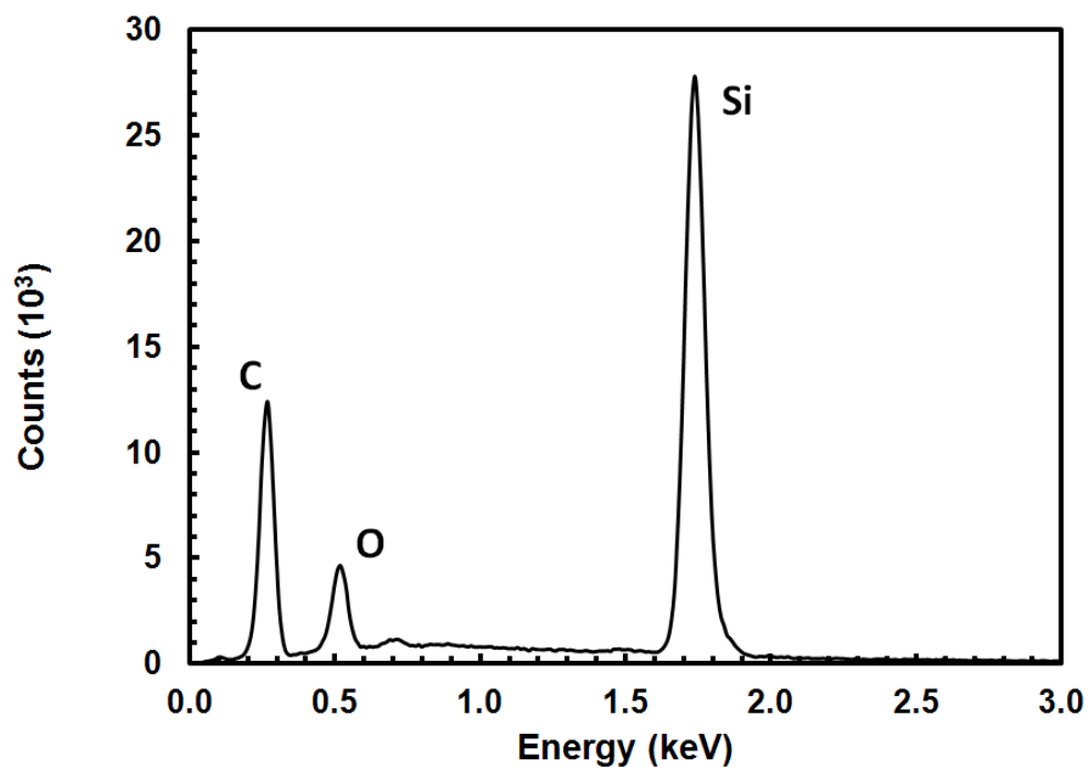
Figure 53. Energy dispersive spectrograph representative of the darker areas of the surface of Hi-Nicalon TM S SiC fiber tow specimen subjected to the saturated steam environment at 800°C and to a load of 2.96 MPa (429.3 psi). The composition is near stoichiometric SiC and a smaller amount of oxygen than the lighter areas. The content was 46.53% silicon, 45.25% carbon, and 7.06% oxygen by atomic percent.
