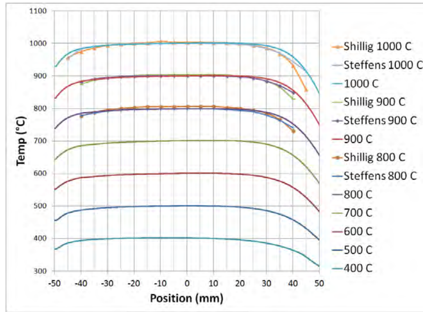
Figure 23. Temperature profiles in air for the current work with data from Steffens [1] and Shillig [23] for comparison.
