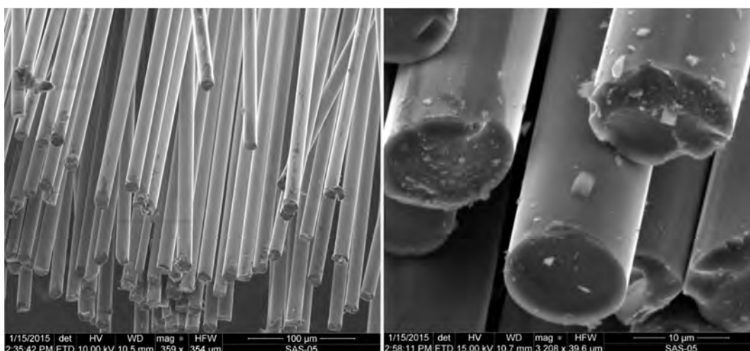
Figure 51. Upper section of Hi-Nicalon TM S SiC fiber tow specimen subjected to the saturated steam environment at 800°C and to a load of 2.96 MPa (429.3 psi)
