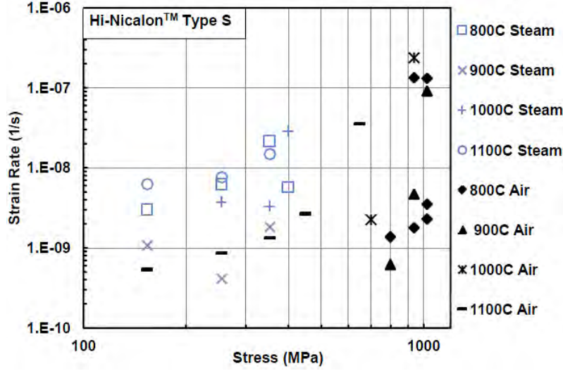
Figure 19. Creep of Hi-Nicalon TM S fibers at 800-1100°C in air and in steam. Note the considerable scatter in the data, making a reliable estimate of the stress exponents impractical. Reproduced from [23].
