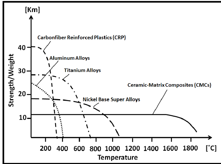
Figure 4. Strength-to-weight ratios of engineering materials for aerospace applications. Note the significant improvement of CMCs over traditional materials at high temperatures. Reproduced from [13], pg. 410, Copyright ©2004, with permission from Elsevier and from the original author [14].
