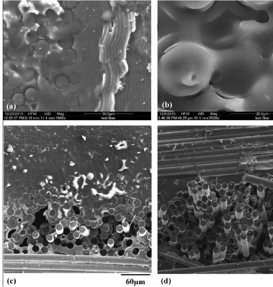
Figure 10. Environmental Degradation due to Oxidation in a SiC/BN/SiC CMC. SEM images showing: (a) oxidation of fibers and matrix, (b) glassy phase in the oxidized region, (c) oxidized region in the top half of the image transitioning to the non-oxidized region in the bottom half of the image, and (d) fiber pull-out typical of the non-oxidized region. Reproduced from [30].
