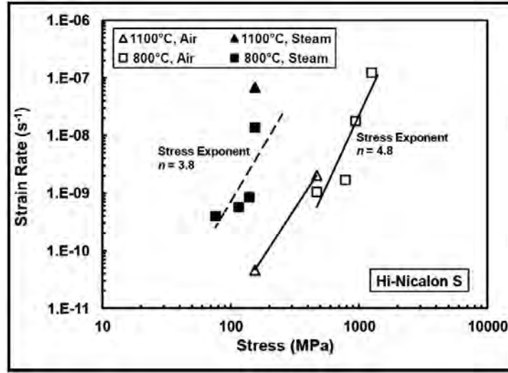
Figure 18. Creep of Hi-Nicalon TM S fibers at 800 and 1100°C in air and in steam, reproduced from [1]
