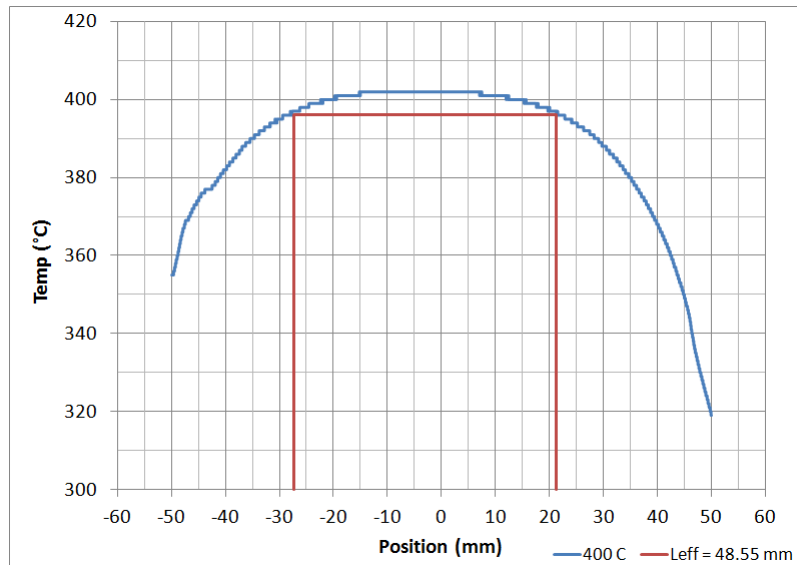
Figure A.8. Effective gauge length and temperature profile in silicic acid saturated steam for 400°C.
