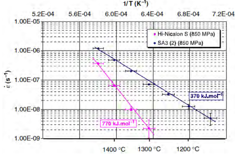
Figure 17. Creep of Tyranno TM SA3 and Hi-Nicalon TM S fibers at 850 MPa (123 ksi)[138], reproduced with permission from Wiley.
