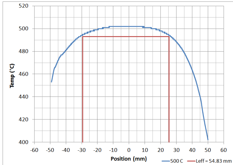
Figure A.9. Effective gauge length and temperature profile in silicic acid saturated steam for 500°C.
