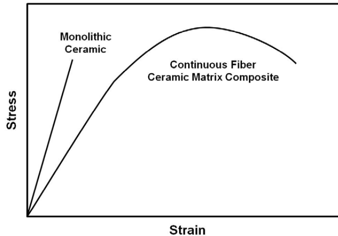
Figure 3. Notional comparison of stress-strain behaviors of a monolithic ceramic and a CMC, reproduced from [4]
