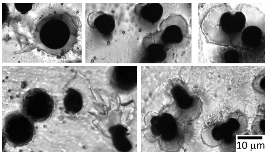
Figure 77. Optical micrograph of Hi-Nicalon TM S fiber tow specimen subjected to oxidation for 100 h at 800°C [198], used with permission.
