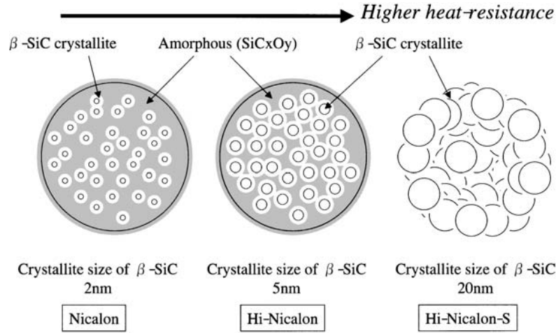
Figure 12. Microstructures of three generations of Nicalon TM fibers. Reproduced with kind permission from Springer Science & Business Media B.V. [20] pg. 118, Figure 9. Copyright ©2005 by Springer-Verlag Berlin Heidelberg.
