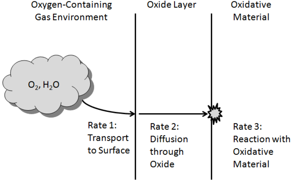
Figure 70. Schematic of oxidation dependence on mass transport, diffusion, and reaction rates.
