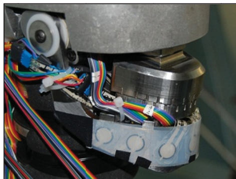
Figure 2: Discrete TekScan FlexiForce® sensors installed on the MLSH jaw.
