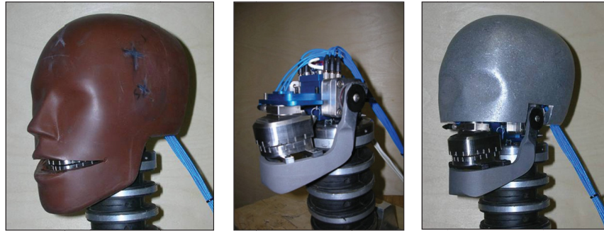
Figure 1: Mandible Load Sensing Headform.
