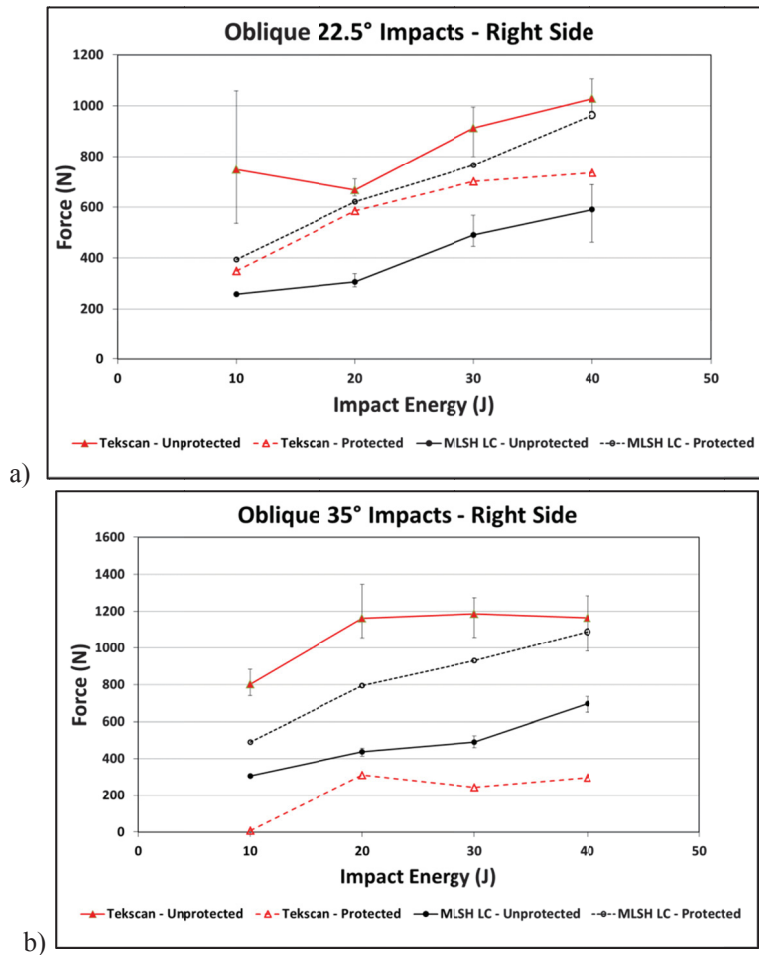
Figure 12: Lateral right 22.5° and 35° right blunt impact test results.
