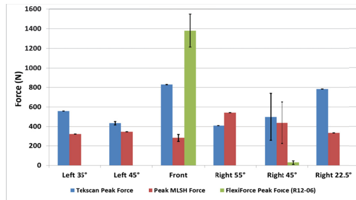
Figure 14: Results of non-penetrating ballistic impacts.
