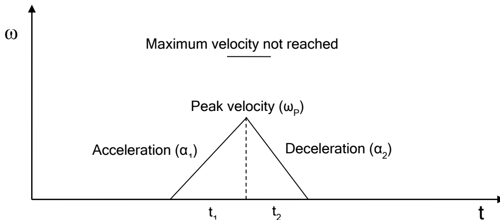
Figure 2 Triangular motion profile
