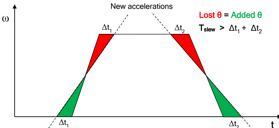
Figure 3 Trapezoidal time adjustment
