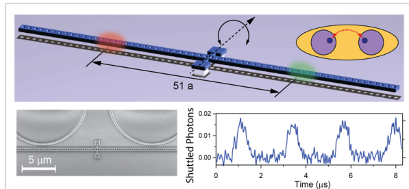
Figure 2 A cavity optomechanical photon “see-saw”. Photon shuttling between two photonic crystal cavities was demonstrated. The trace in the lower-right panel shows photons being mechanically shuttled from one cavity to the other.
