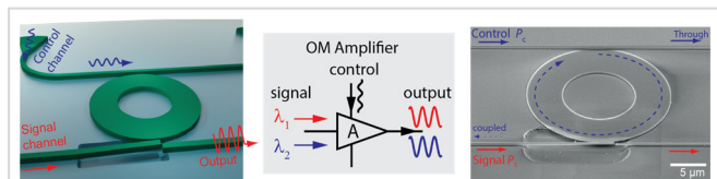
Figure 1 A multichannel cavity optomechanical relay that can amplify radio-frequency signal.
