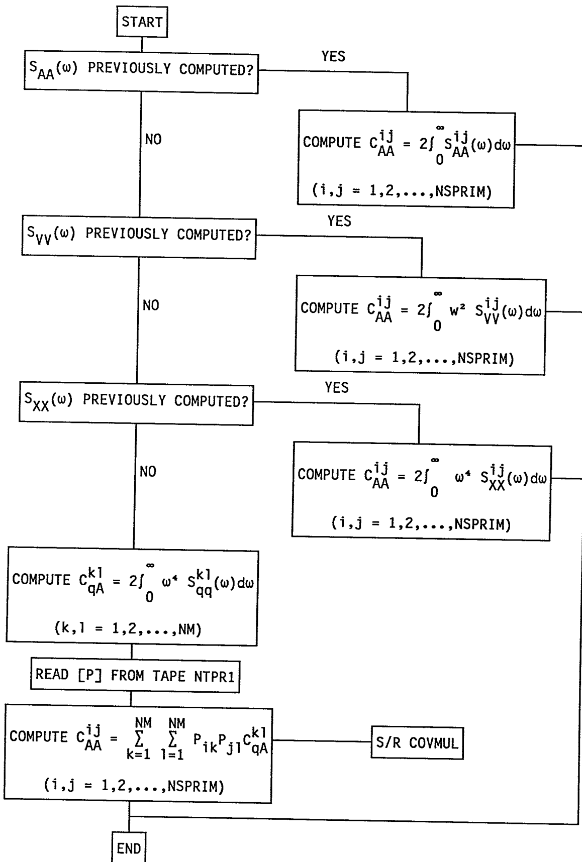
Figure 4.7c. Flow Diagram for the Computation of the Covariance Matrix of Accelerations in Subroutine COVMUL
