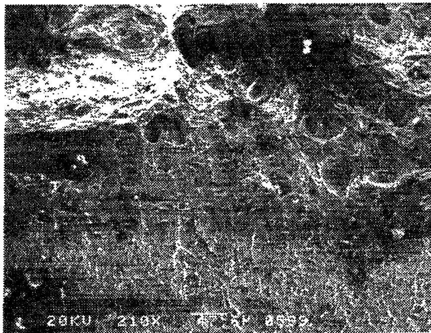
FIGURE A.60: Specimen 15, Position 4 (210 X).
