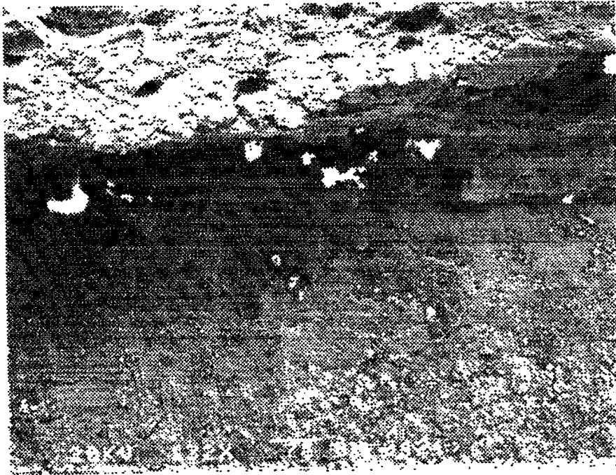
FIGURE A.55: Specimen 14, Position 3 (132 X).
