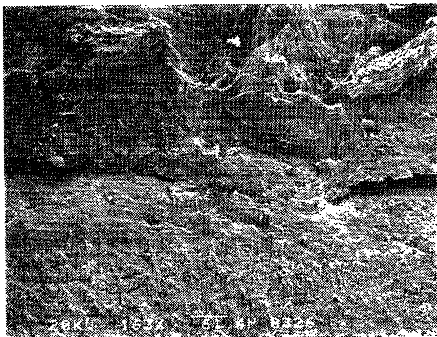
FIGURE A.47: Specimen 12, Position 3 (163 X).
