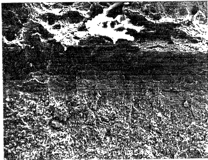
FIGURE A.72: Specimen 21, Position 4 (270 X).
