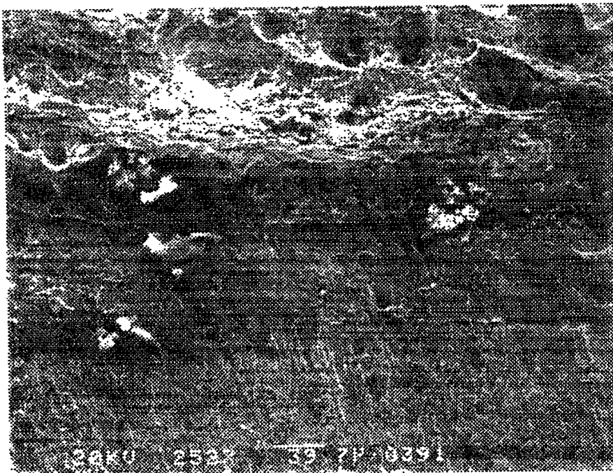
FIGURE A.24: Specimen 6, Position 4 (252 X).
