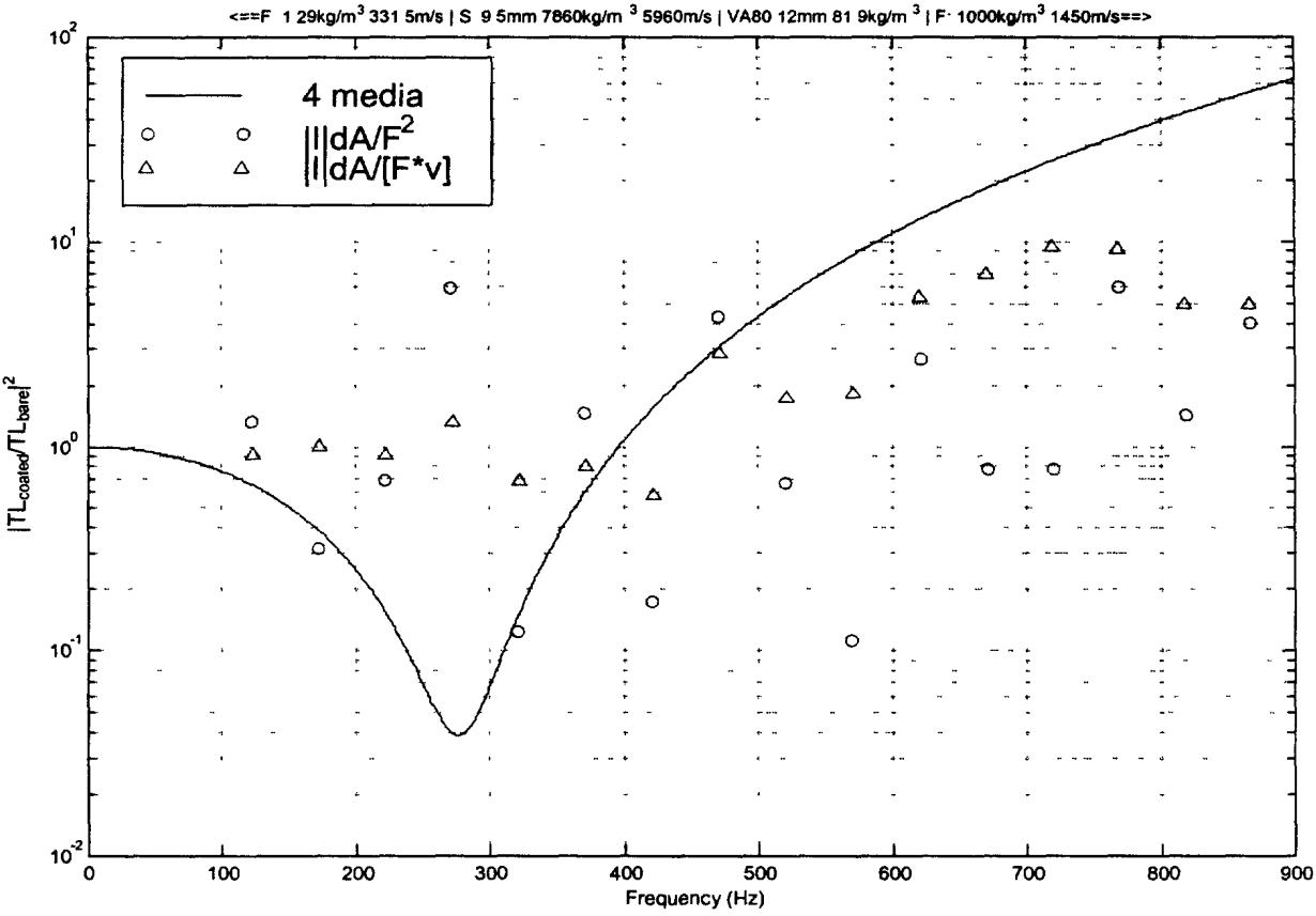
Decoupling Performance: 12mm VA80 on 9.5mm plate
