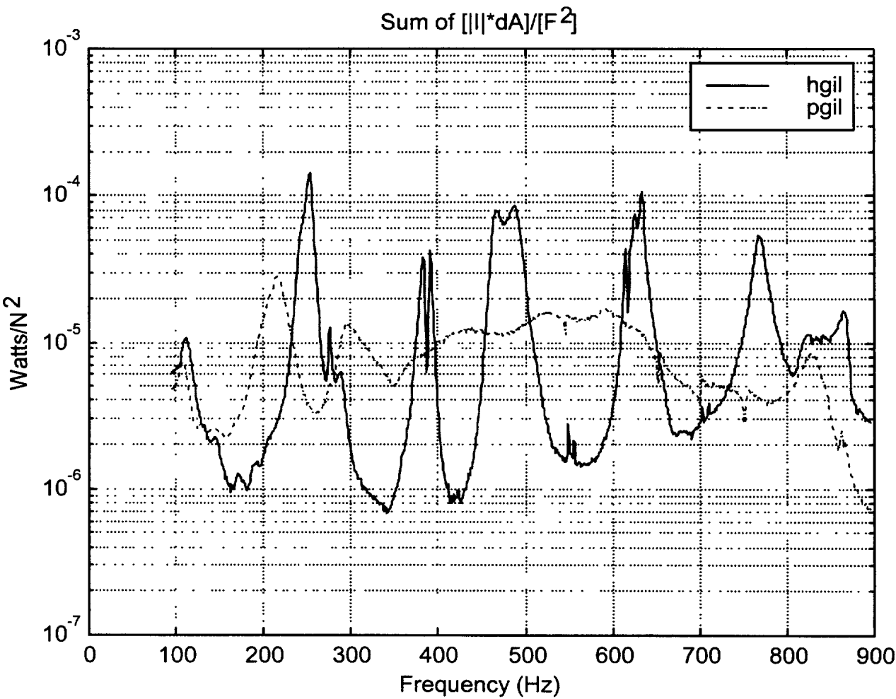
Plate H (9.5 mm bare steel) vs Plate P (9.5 mm steel 12 mm VA80)
