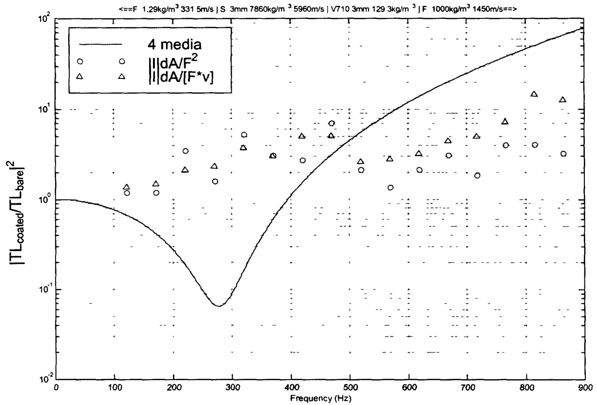
Decoupling Performance: 3mm V710 on 3mm plate
