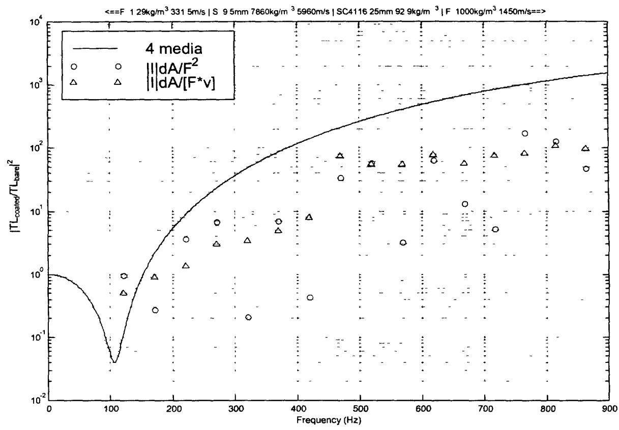
Decoupling Performance: 25mm SC4116 on 9.5mm plate
