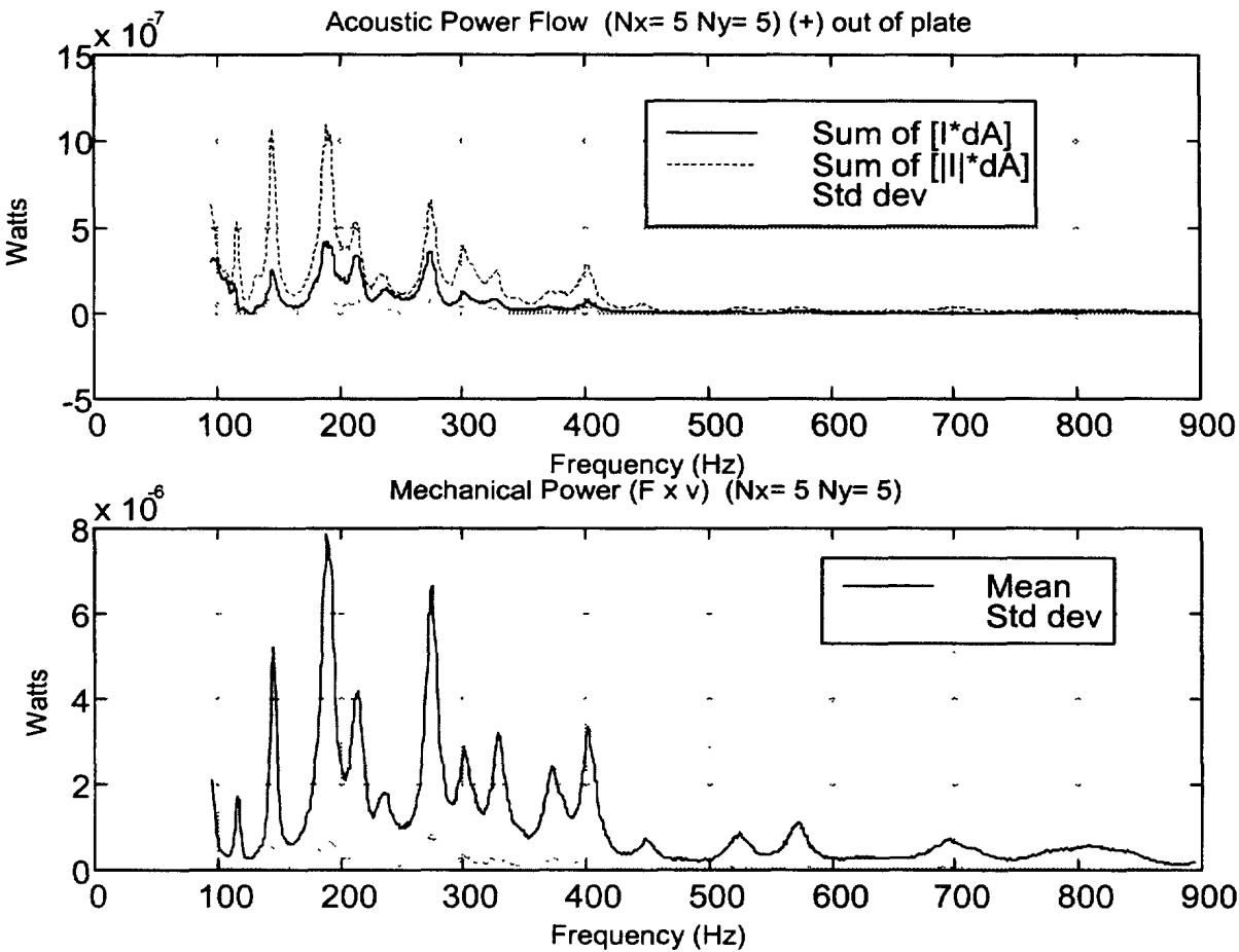
Plate M: 3 mm steel plate coated with 3 mm C-1002
