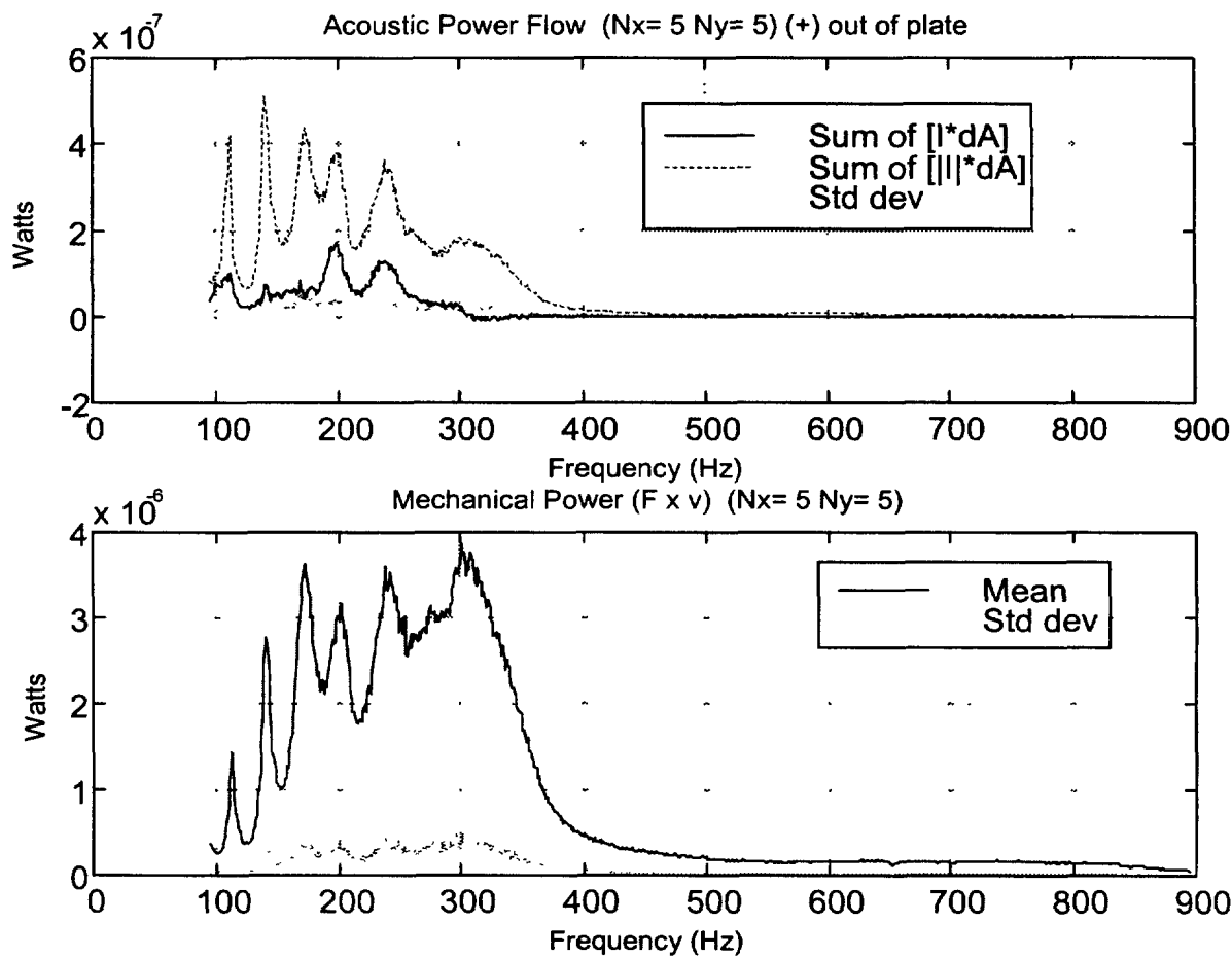
Plate Q: 3 mm steel plate coated with 23 mm VA80 foam
