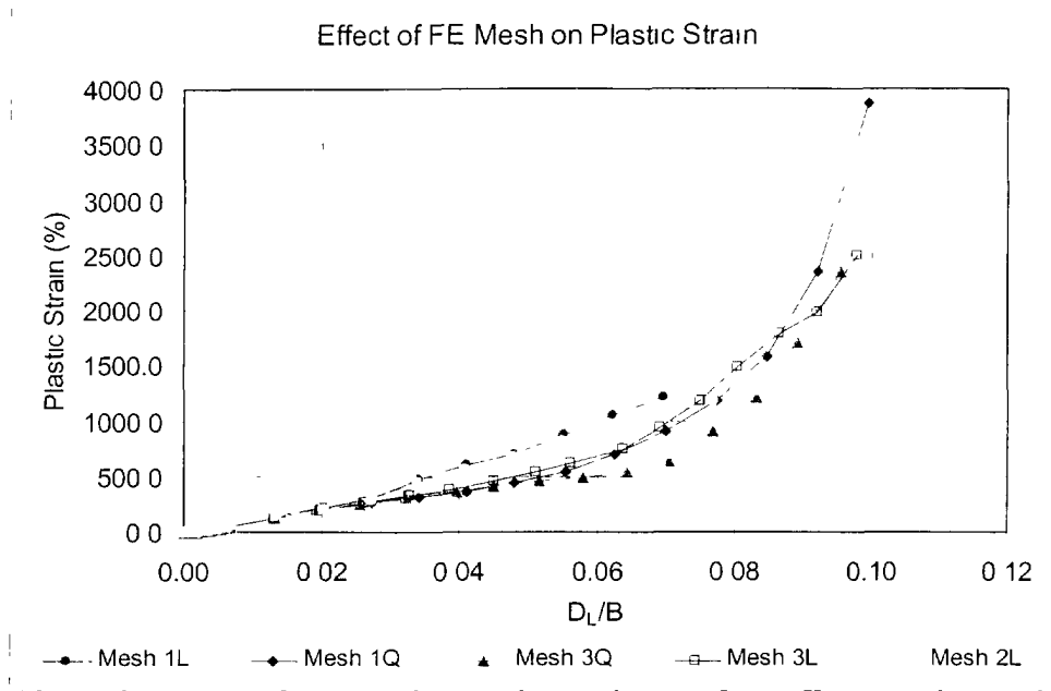
Figure 4.8: Variation of Maximum Plastic Strain with Non-Dimensionalized Displacement for all Specimens
