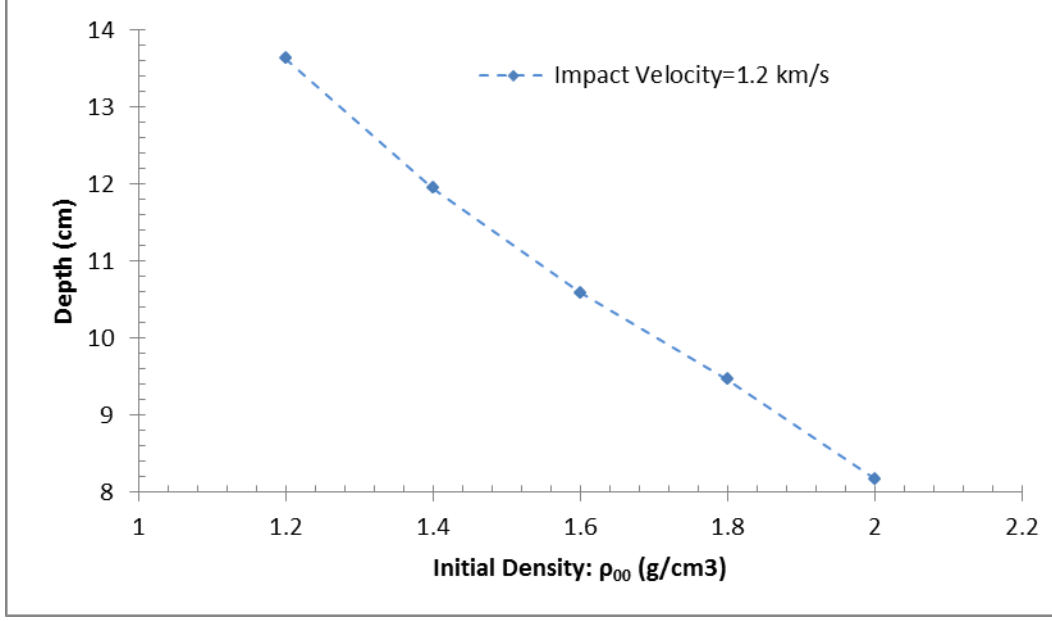
Figure 15: Penetrator Depth versus Density of Computational Data varying Initial Densities at Constant Impact Velocity
