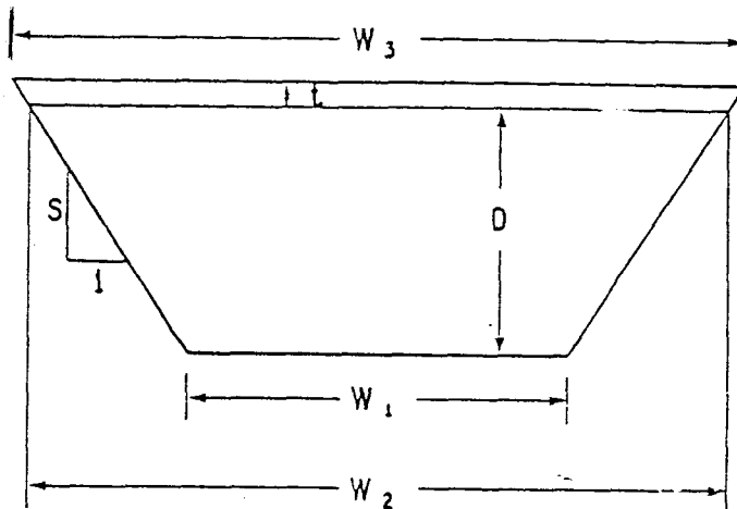
Figure 2. Channel Cross Section
