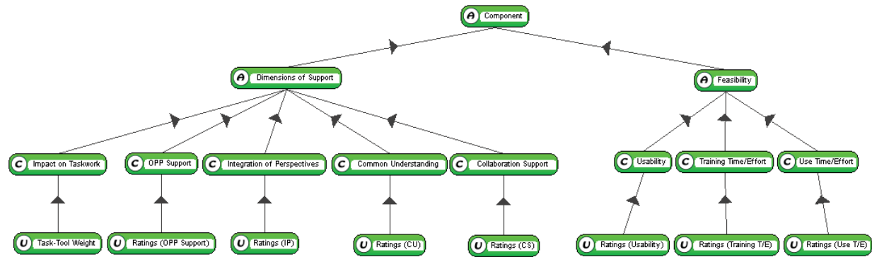
Figure 11: Methodology Component Analysis Using a MYRIAD Preference Model.
